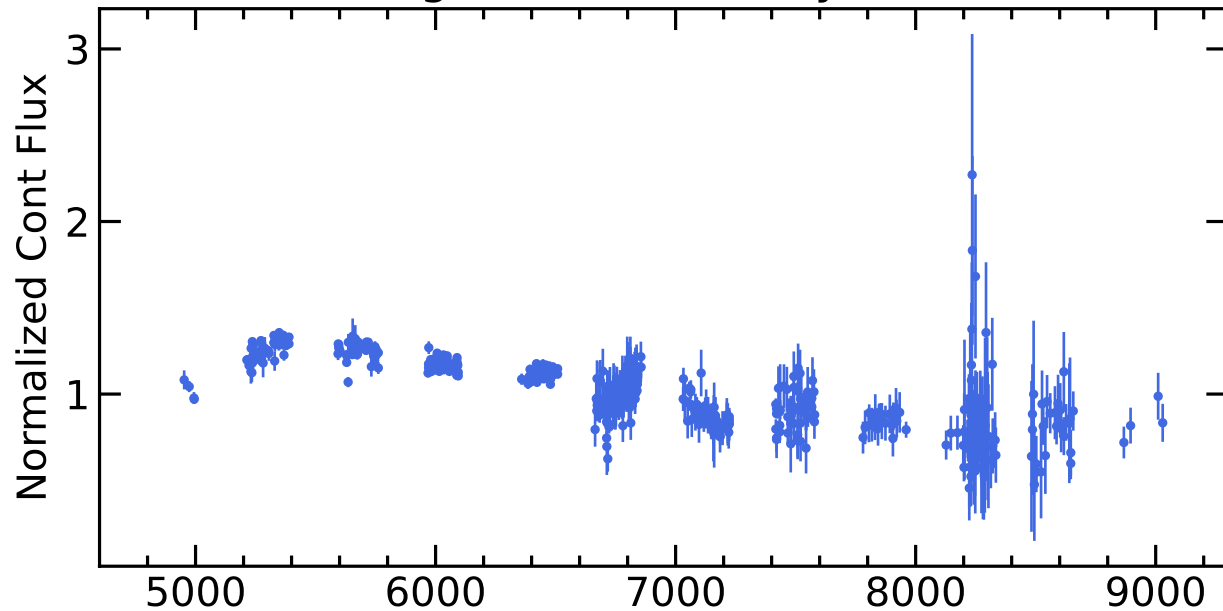
RM661 Light Curves (w/ PyROA model)
