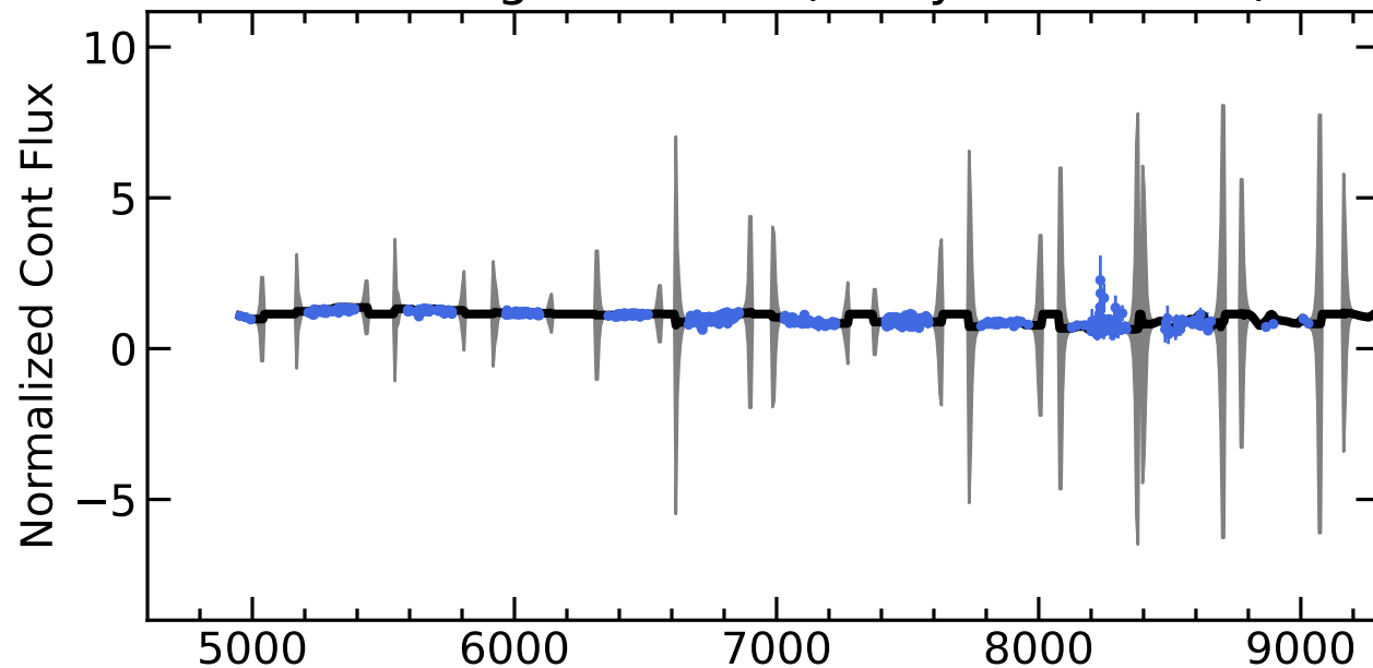
RM661 Light Curves (w/ PyROA model)
