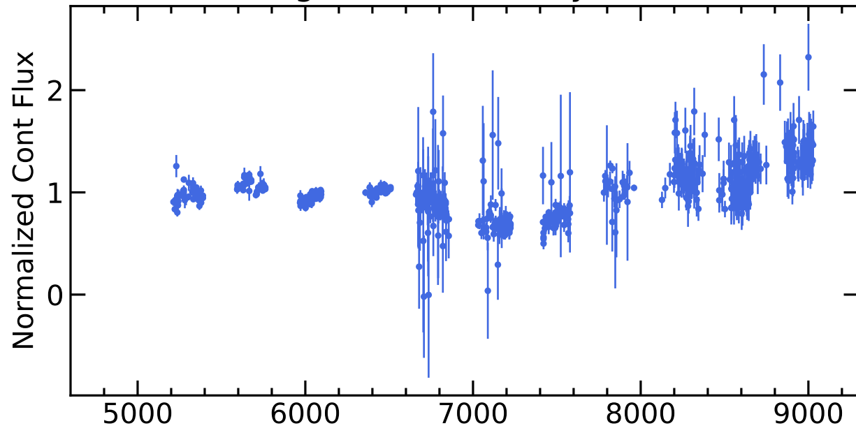
RM662 Light Curves (w/ PyROA model)
