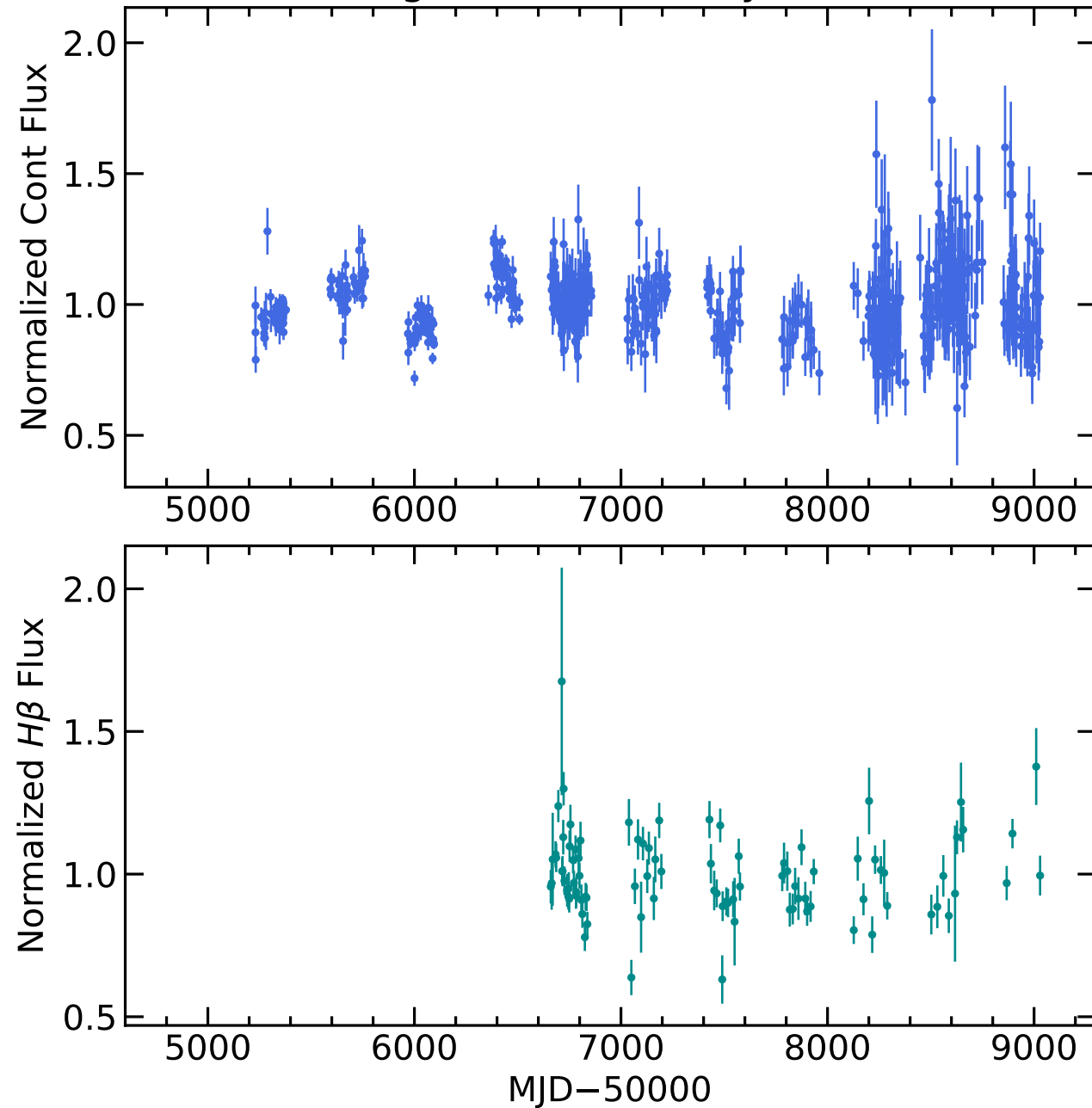
RM663 Light Curves (w/ PyROA model)
