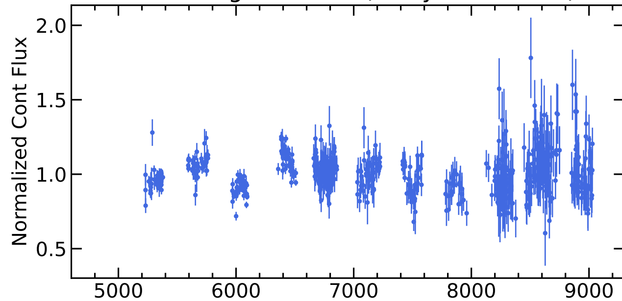
RM663 Light Curves (w/ PyROA model)
