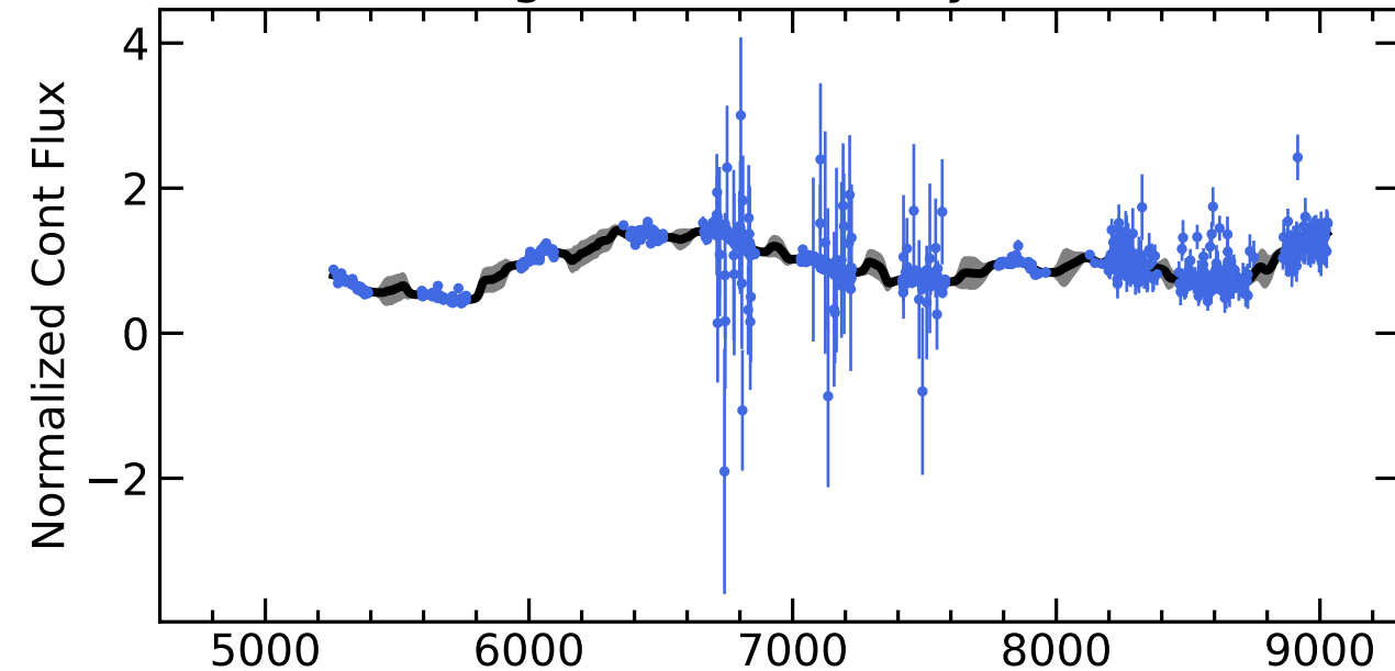
RM664 Light Curves (w/ PyROA model)
