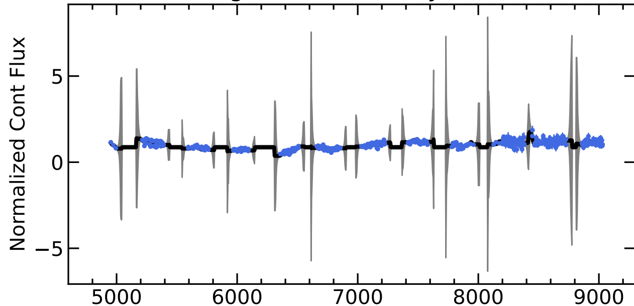
RM665 Light Curves (w/ PyROA model)
