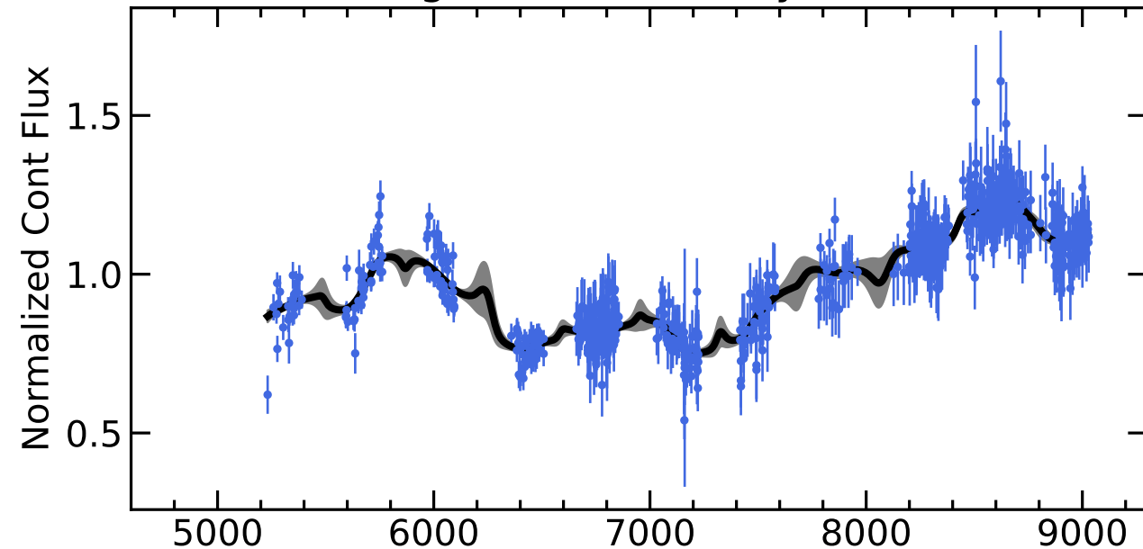
RM666 Light Curves (w/ PyROA model)
