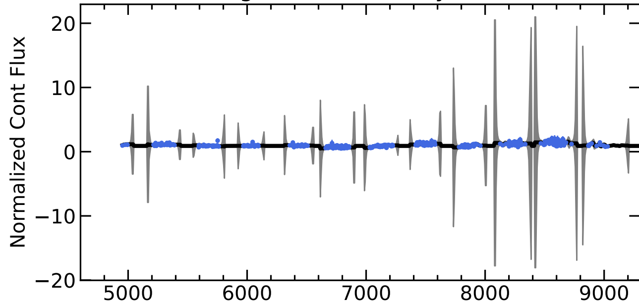
RM667 Light Curves (w/ PyROA model)
