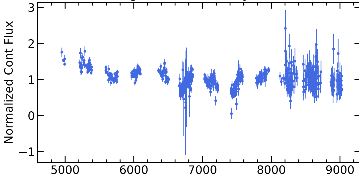
RM668 Light Curves (w/ PyROA model)
