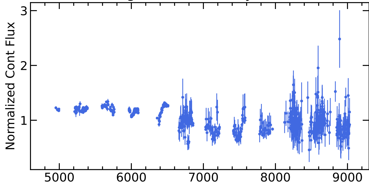
RM669 Light Curves (w/ PyROA model)
