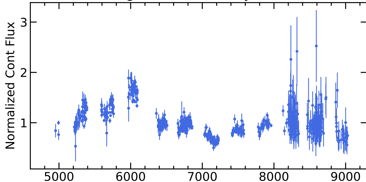
RM670 Light Curves (w/ PyROA model)
