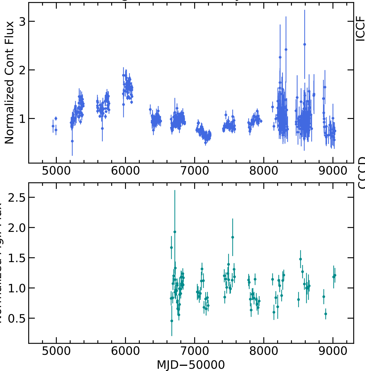
RM670 Light Curves (w/ PyROA model)
