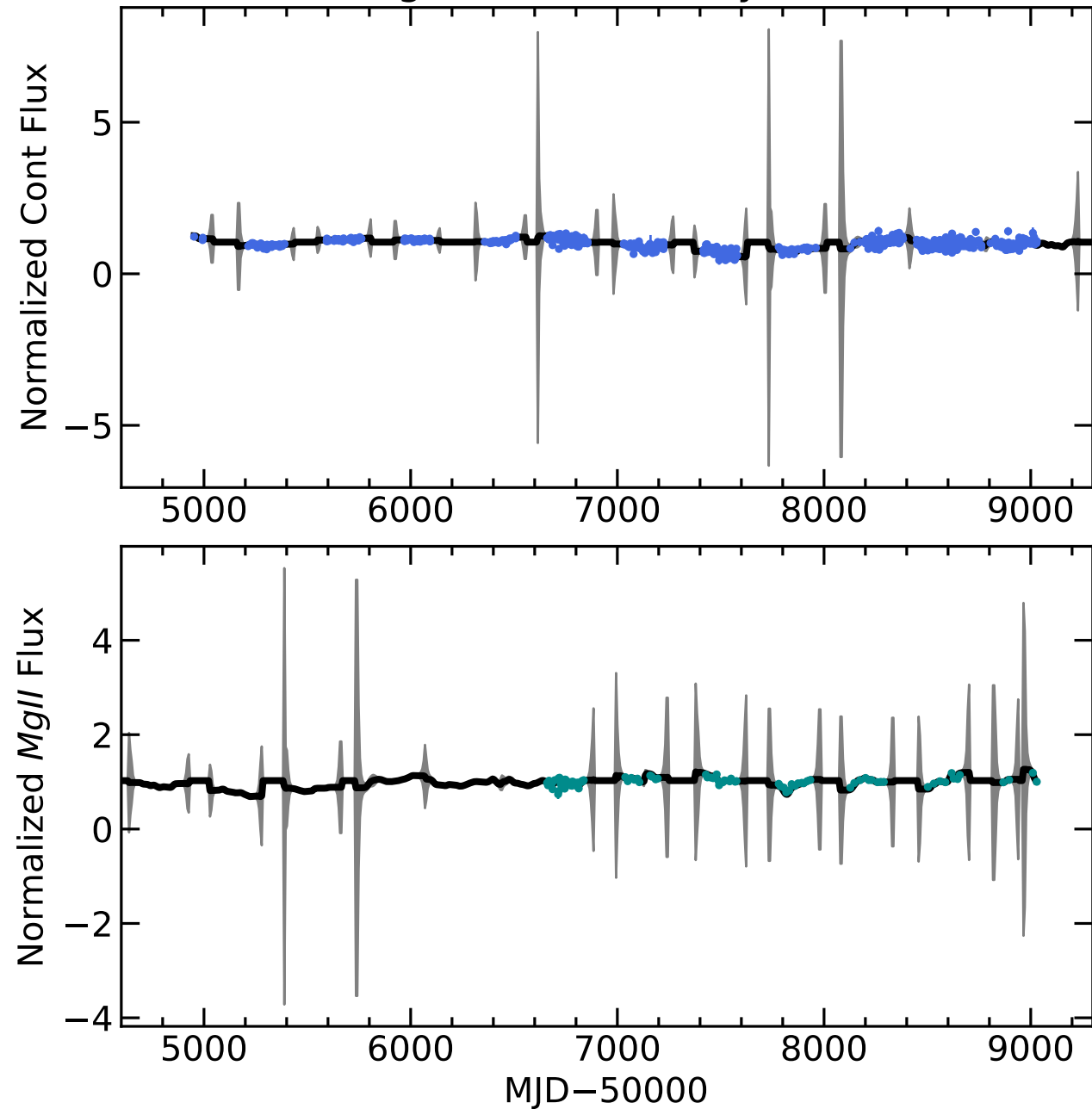
RM671 Light Curves (w/ PyROA model)
