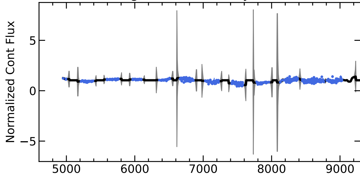
RM671 Light Curves (w/ PyROA model)
