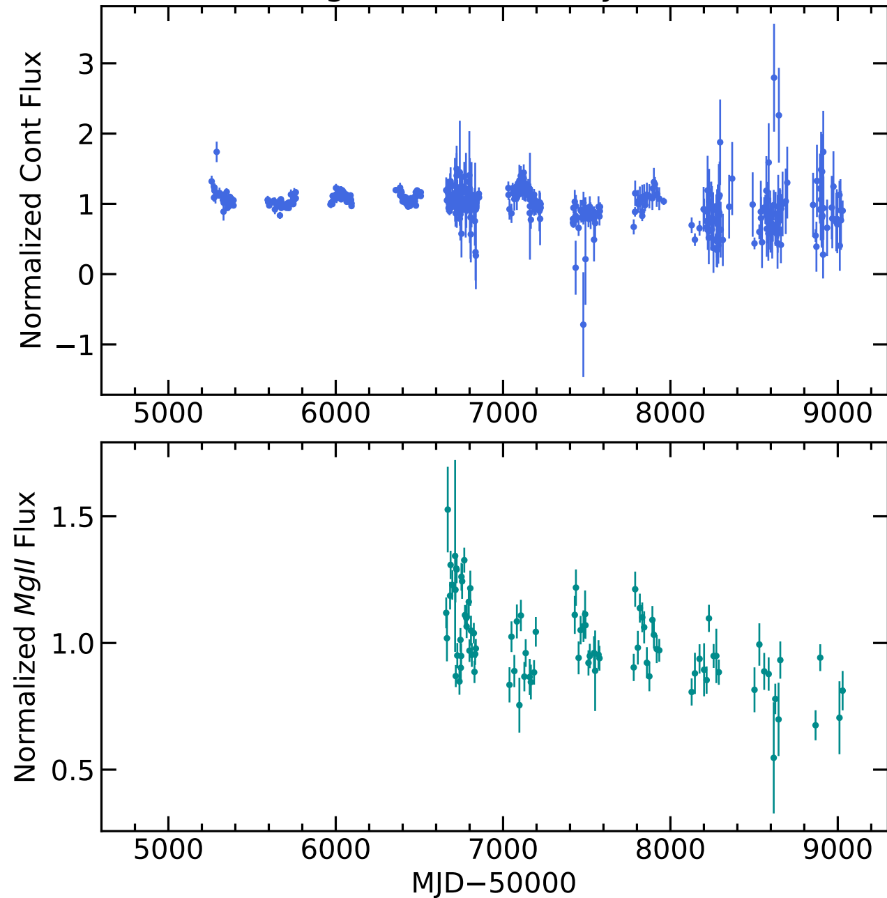
RM672 Light Curves (w/ PyROA model)
