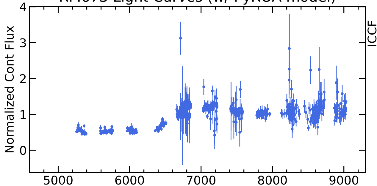
RM673 Light Curves (w/ PyROA model)
