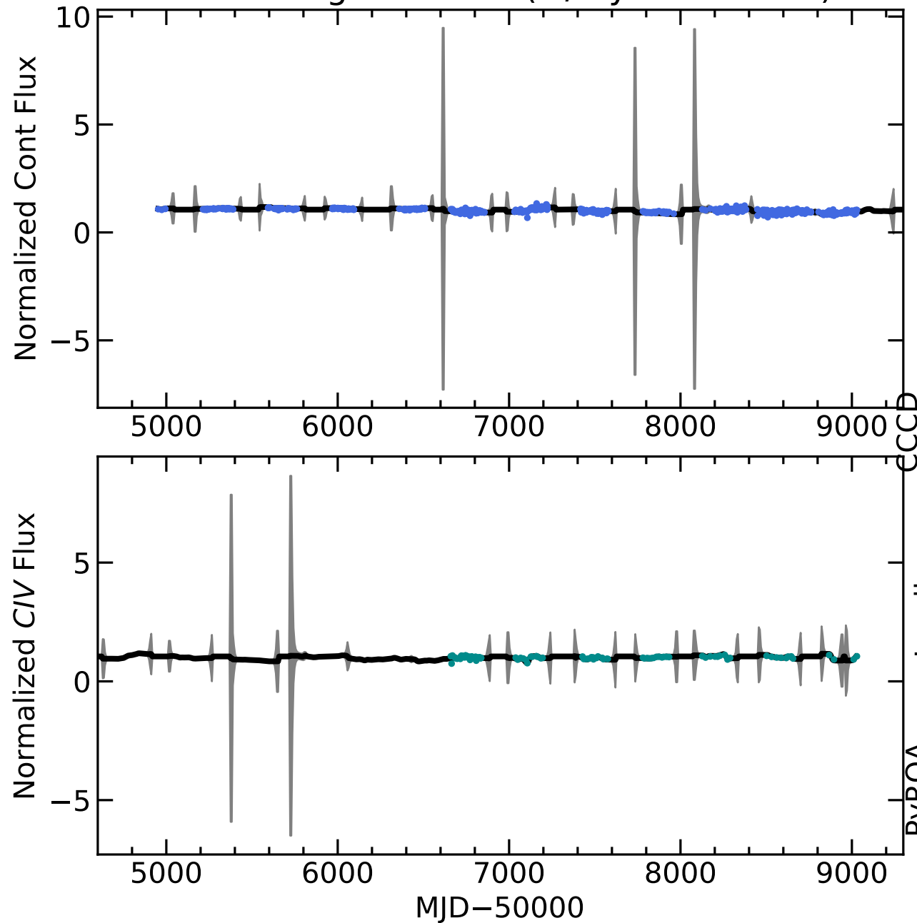
RM676 Light Curves (w/ PyROA model)
