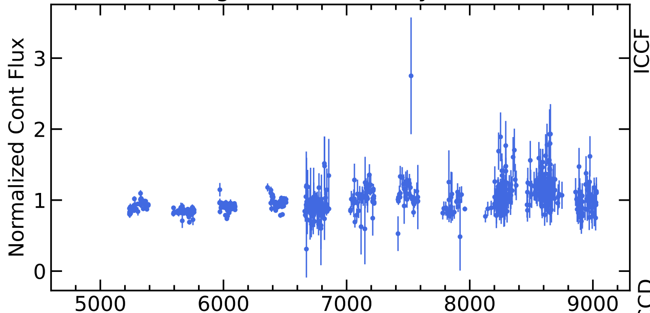
RM677 Light Curves (w/ PyROA model)
