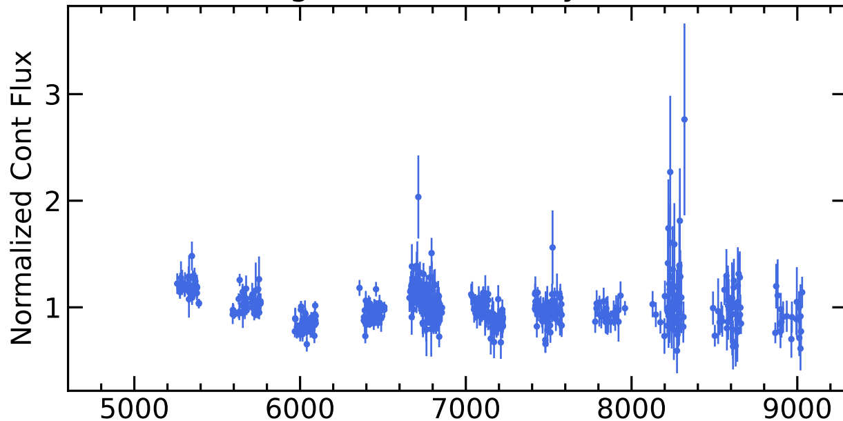
RM679 Light Curves (w/ PyROA model)
