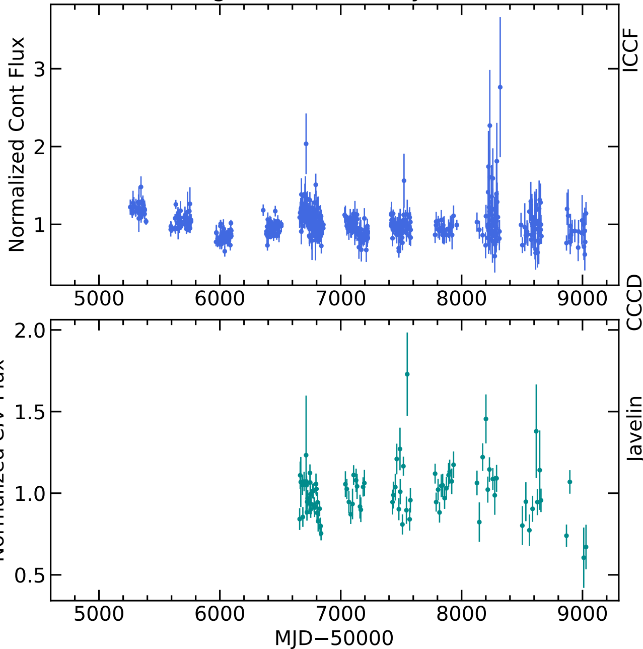
RM679 Light Curves (w/ PyROA model)
