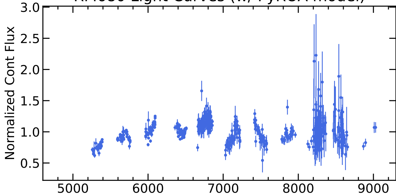
RM680 Light Curves (w/ PyROA model)
