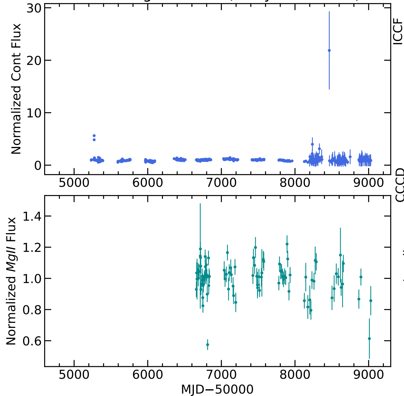
RM681 Light Curves (w/ PyROA model)
