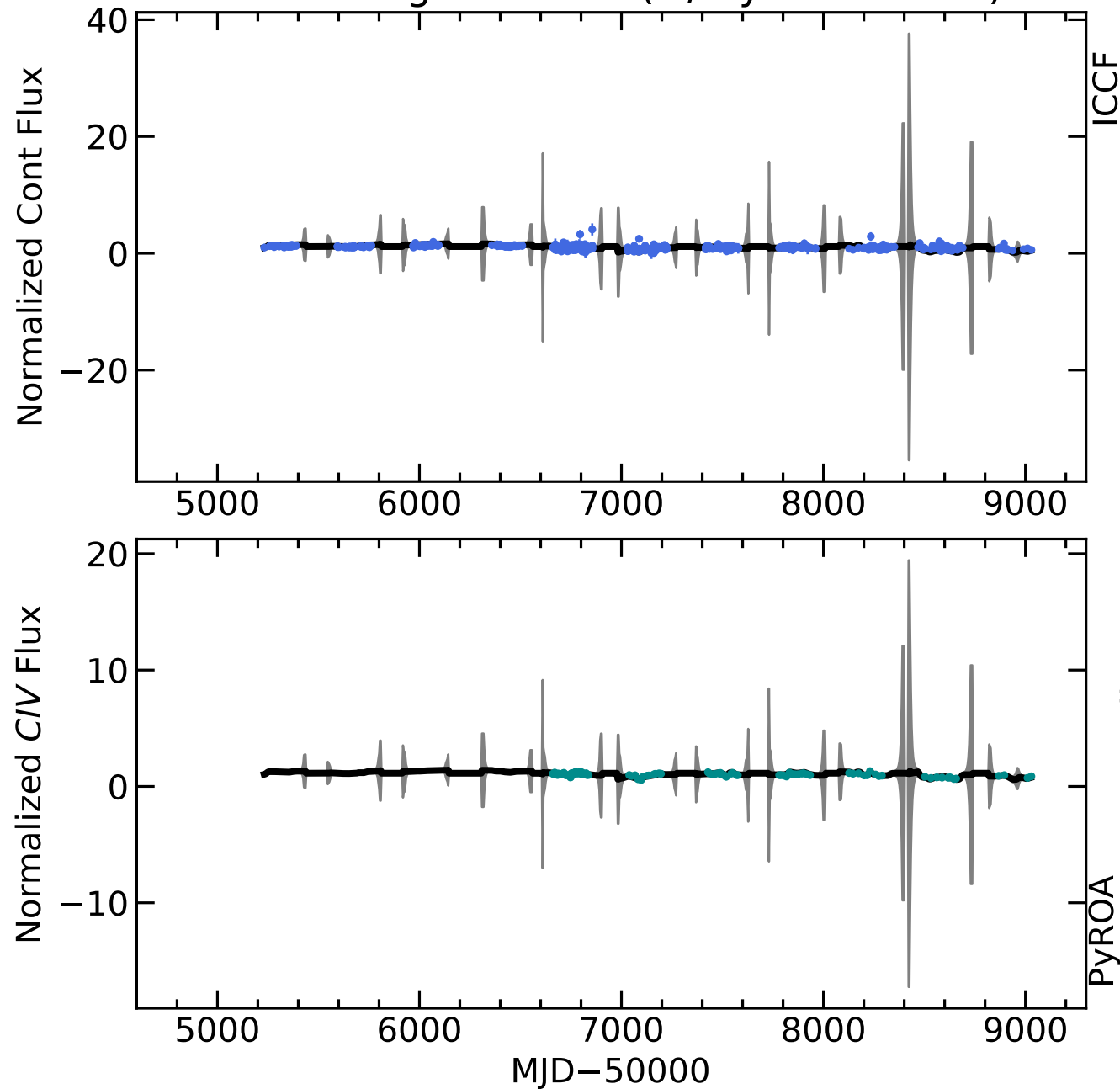
RM682 Light Curves (w/ PyROA model)
