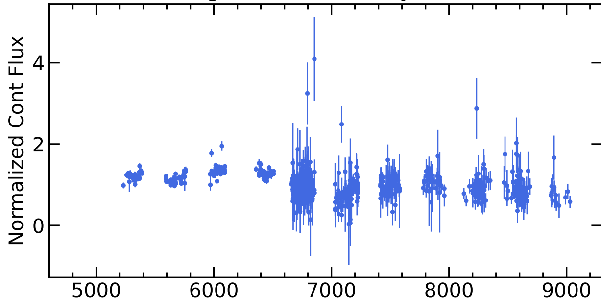
RM682 Light Curves (w/ PyROA model)
