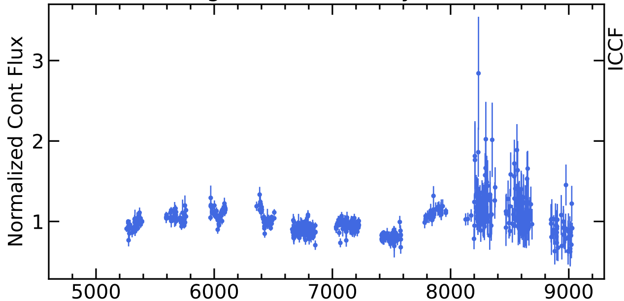
RM683 Light Curves (w/ PyROA model)
