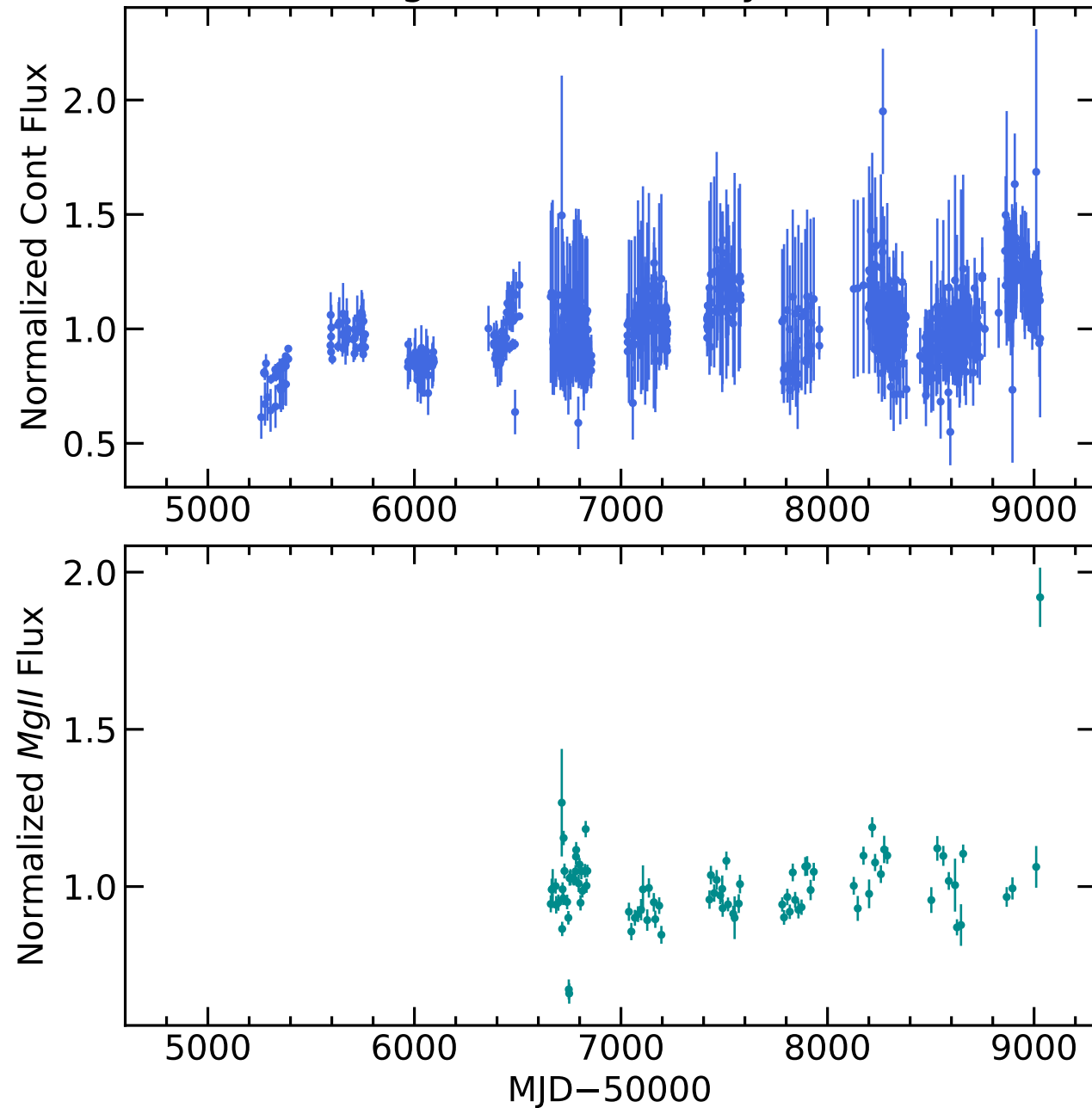
RM685 Light Curves (w/ PyROA model)
