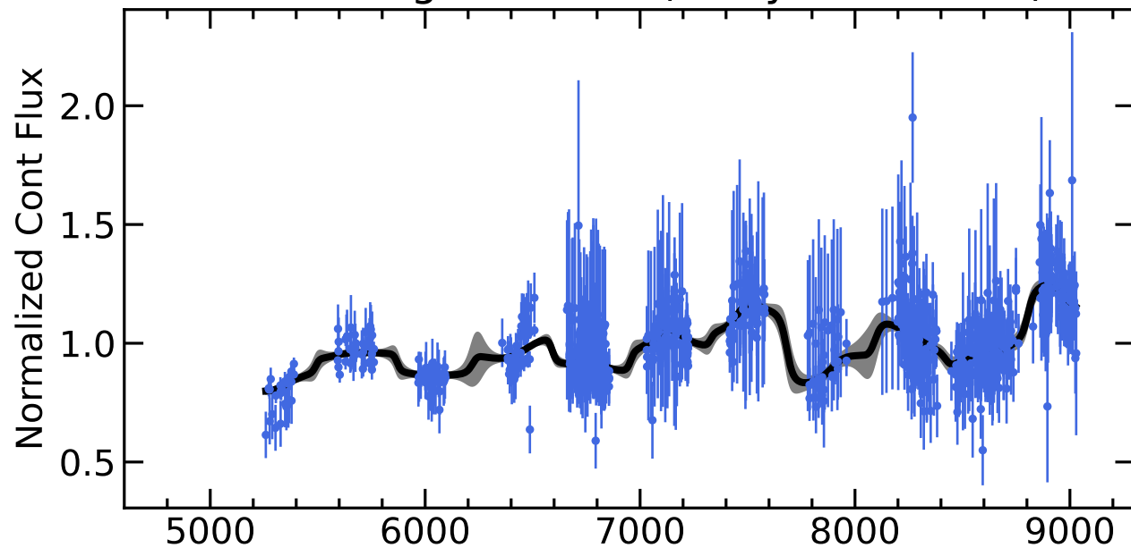
RM685 Light Curves (w/ PyROA model)
