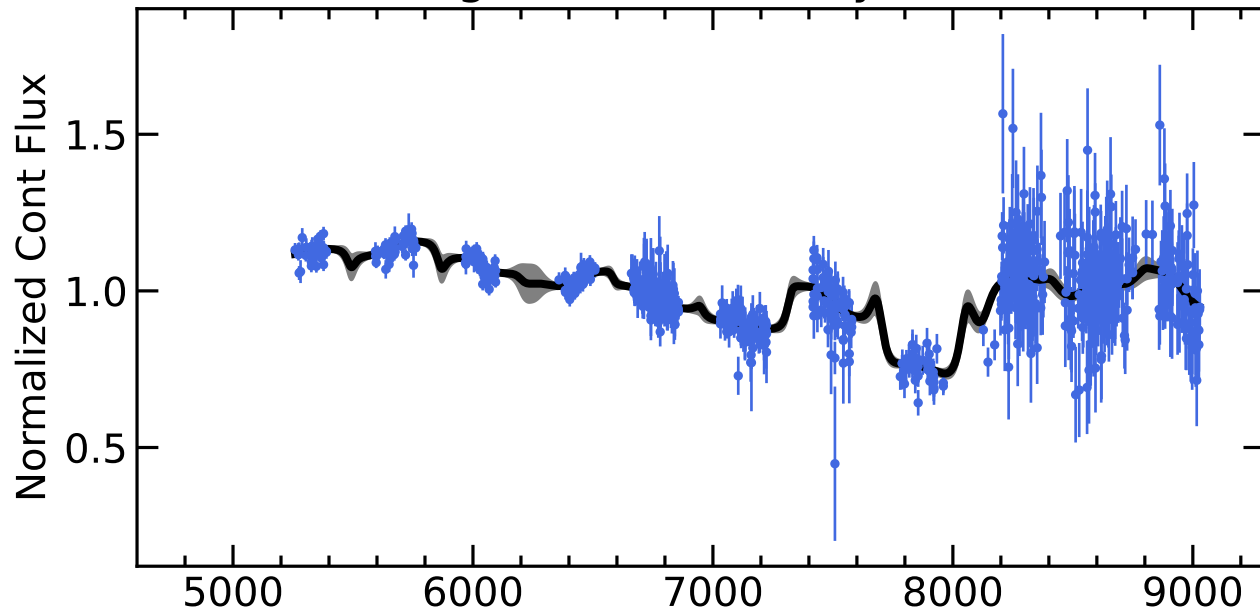
RM688 Light Curves (w/ PyROA model)
