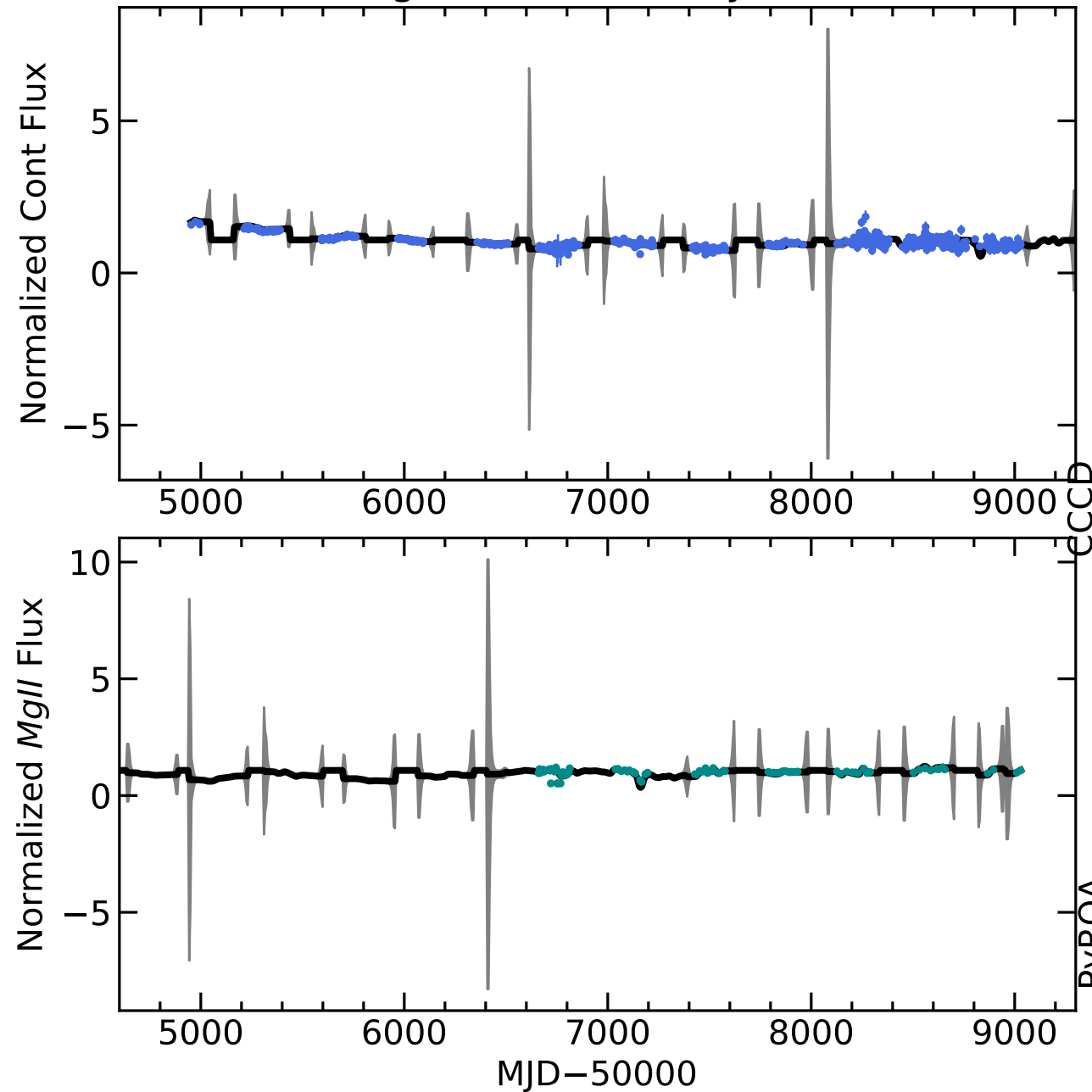
RM690 Light Curves (w/ PyROA model)
