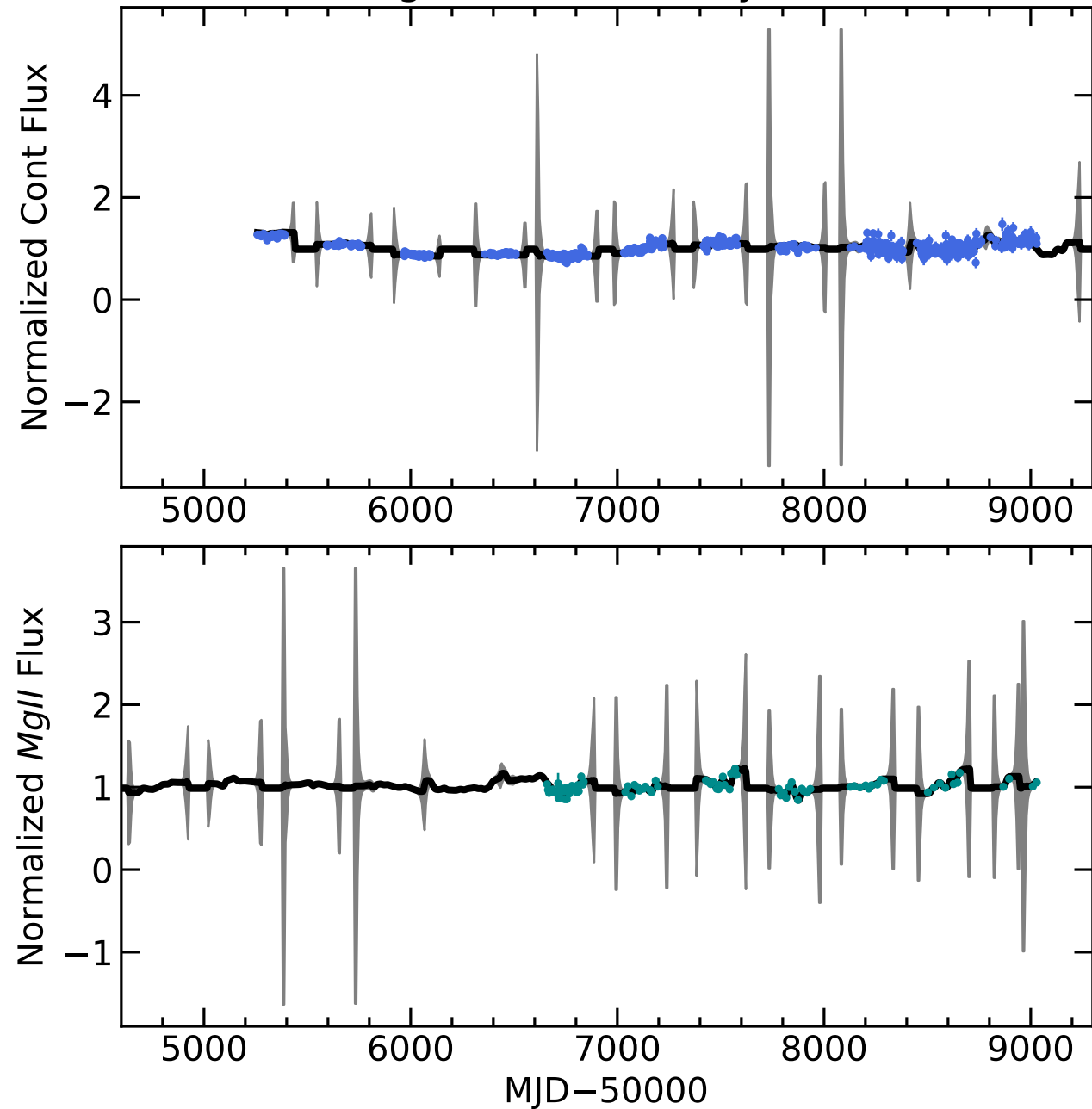
RM692 Light Curves (w/ PyROA model)
