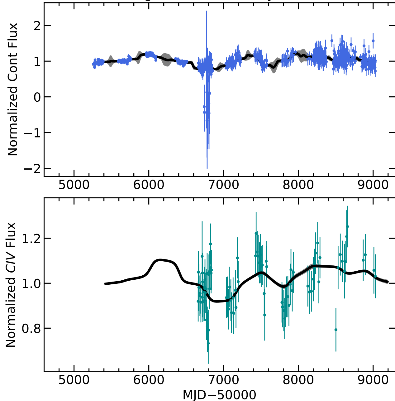
RM693 Light Curves (w/ PyROA model)
