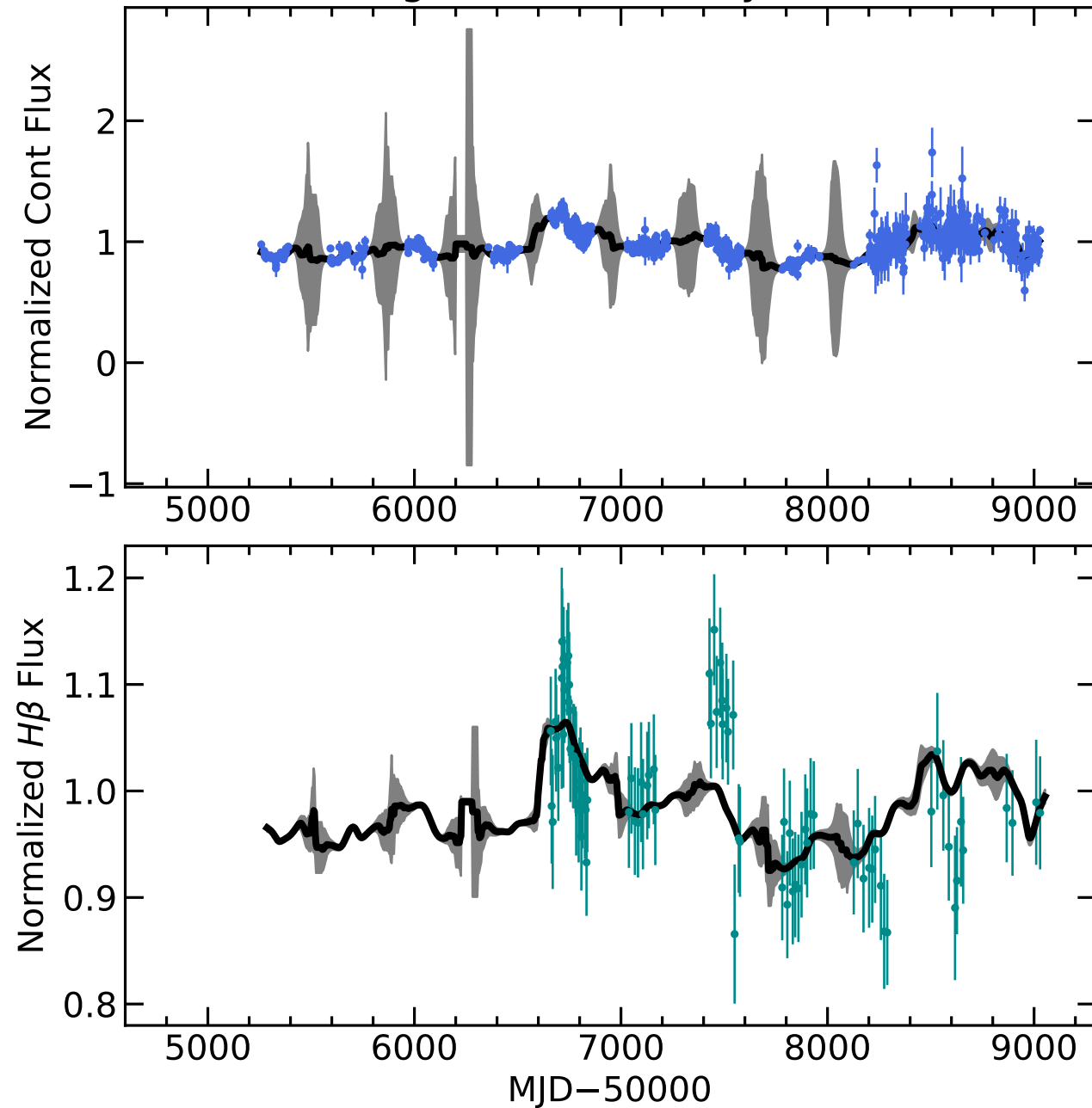
RM694 Light Curves (w/ PyROA model)
