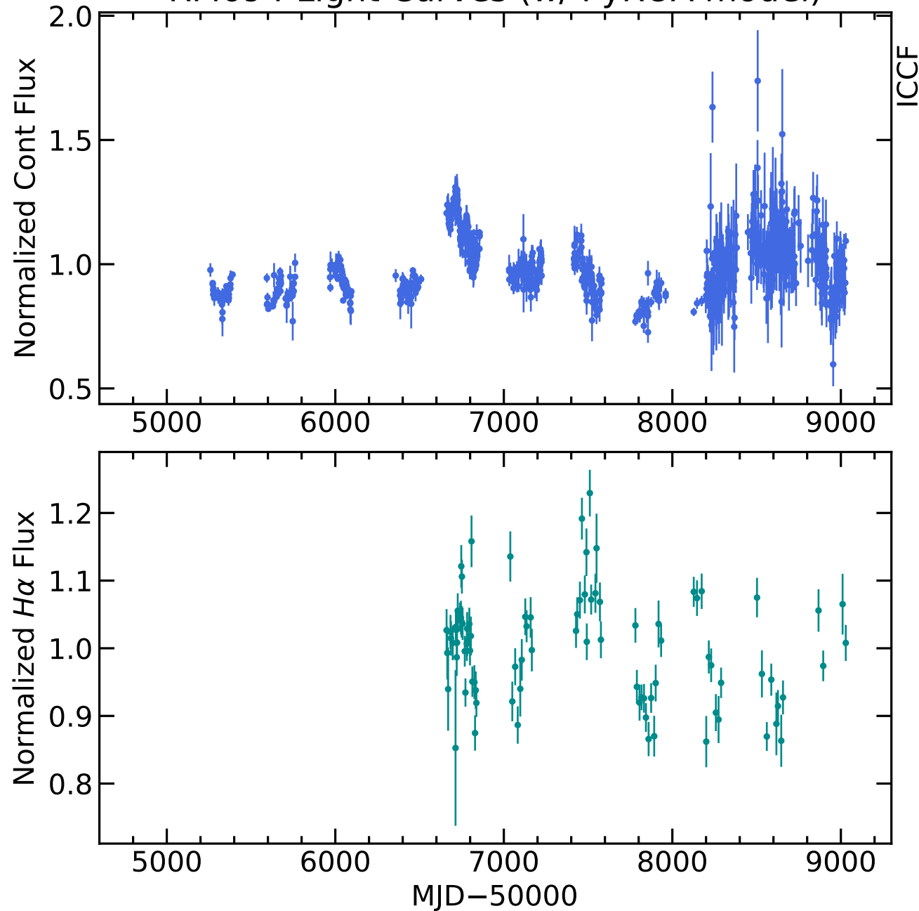
RM694 Light Curves (w/ PyROA model)
