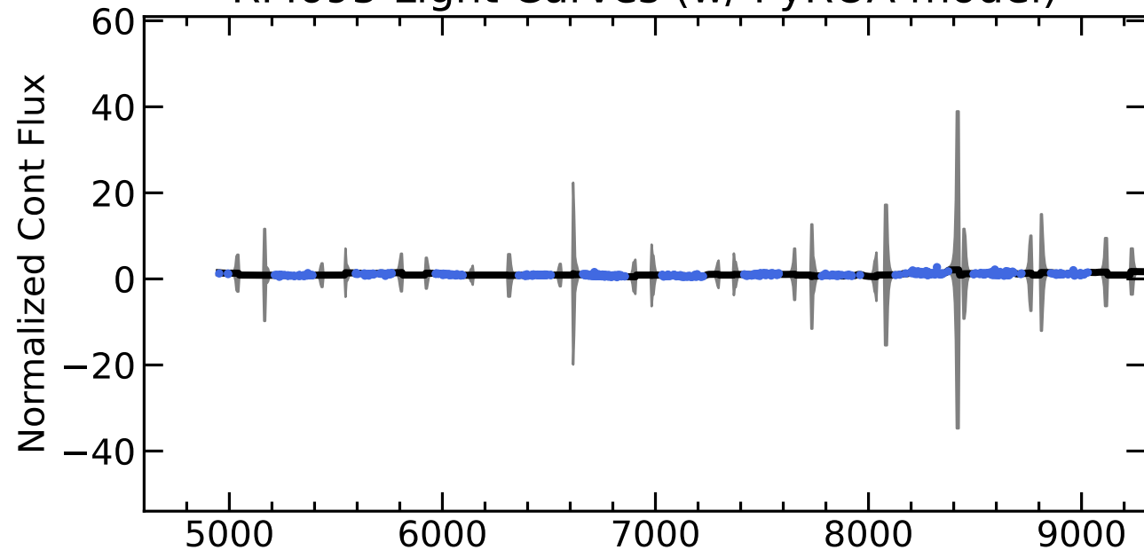
RM695 Light Curves (w/ PyROA model)
