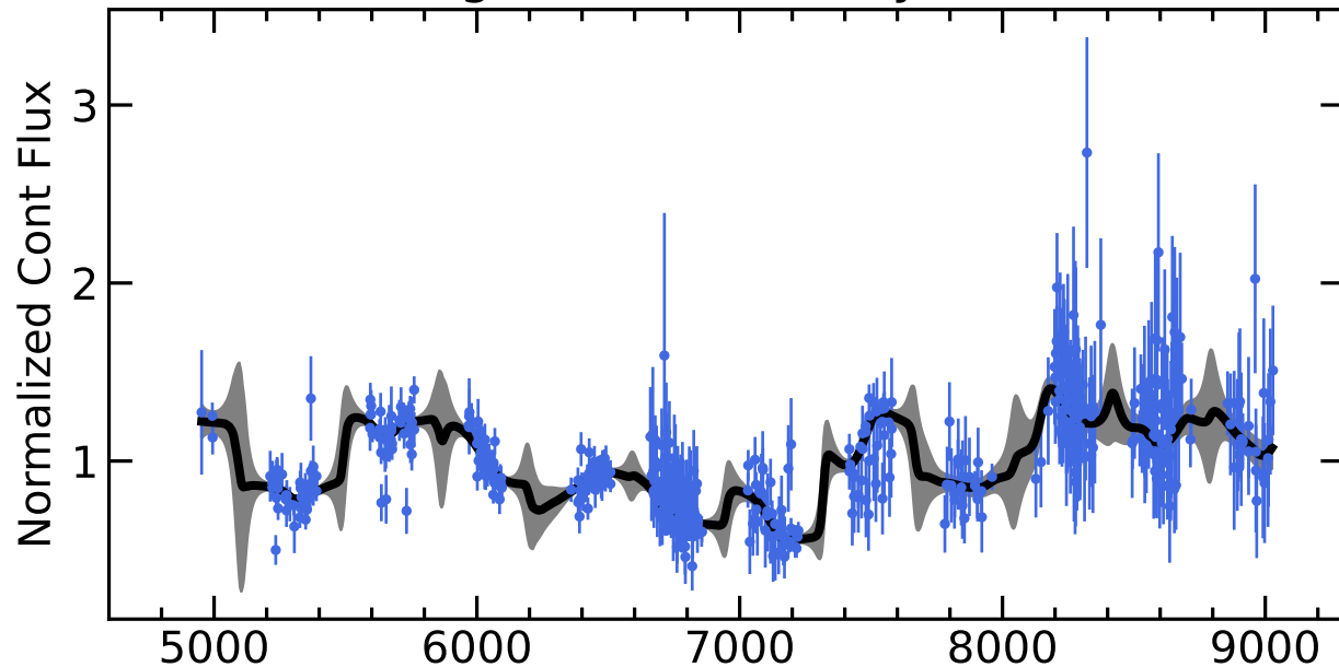
RM695 Light Curves (w/ PyROA model)
