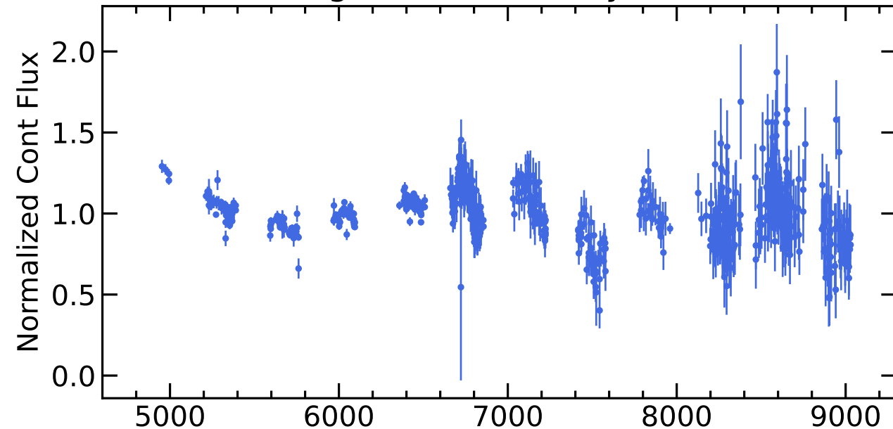
RM696 Light Curves (w/ PyROA model)
