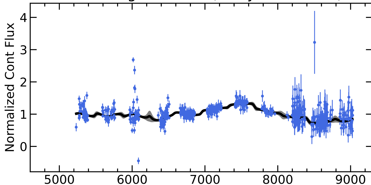
RM698 Light Curves (w/ PyROA model)
