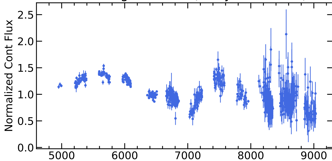
RM699 Light Curves (w/ PyROA model)
