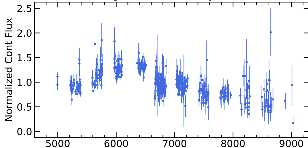
RM700 Light Curves (w/ PyROA model)
