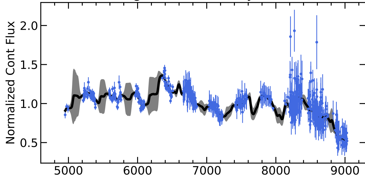
RM701 Light Curves (w/ PyROA model)
