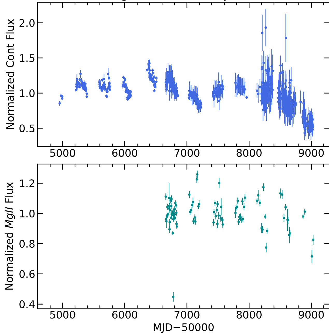
RM701 Light Curves (w/ PyROA model)
