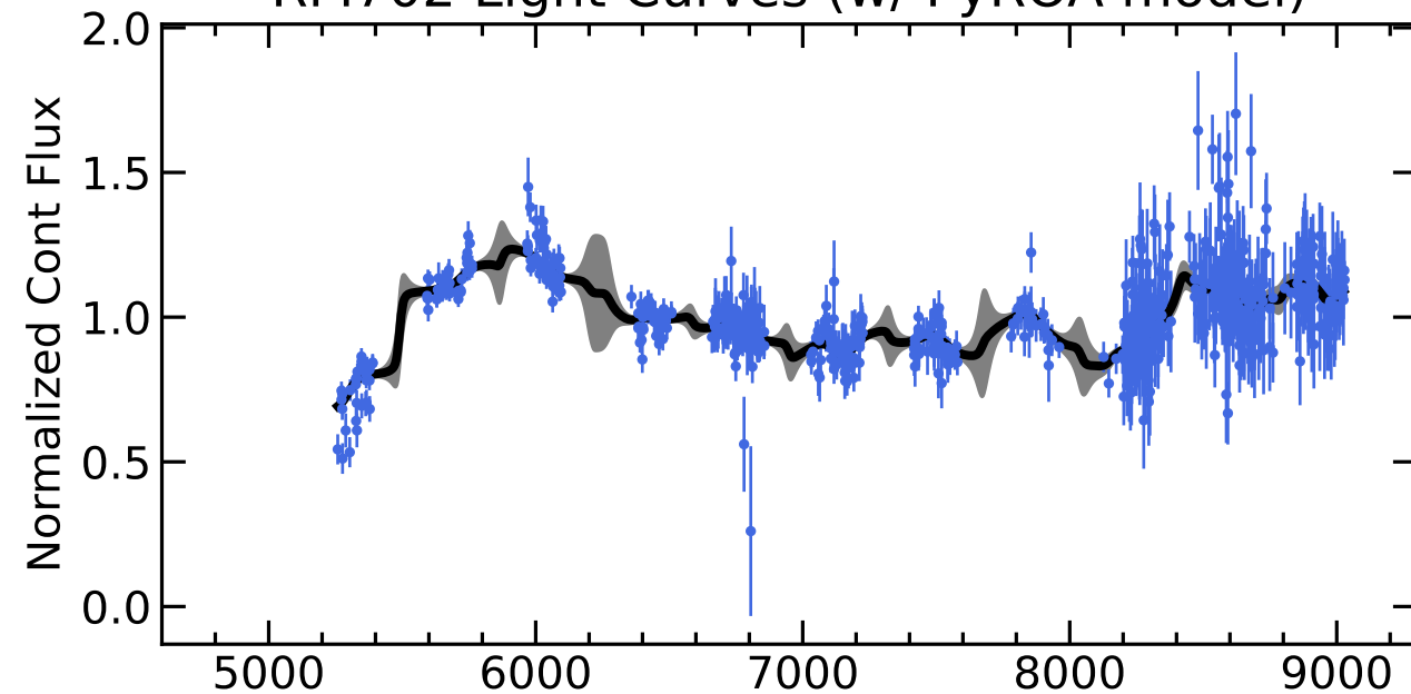
RM702 Light Curves (w/ PyROA model)
