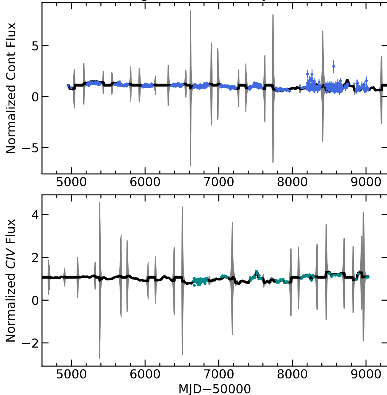
RM703 Light Curves (w/ PyROA model)
