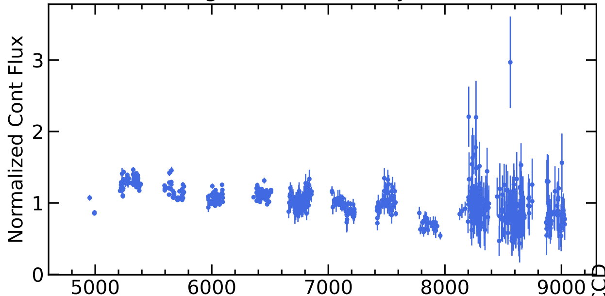
RM703 Light Curves (w/ PyROA model)
