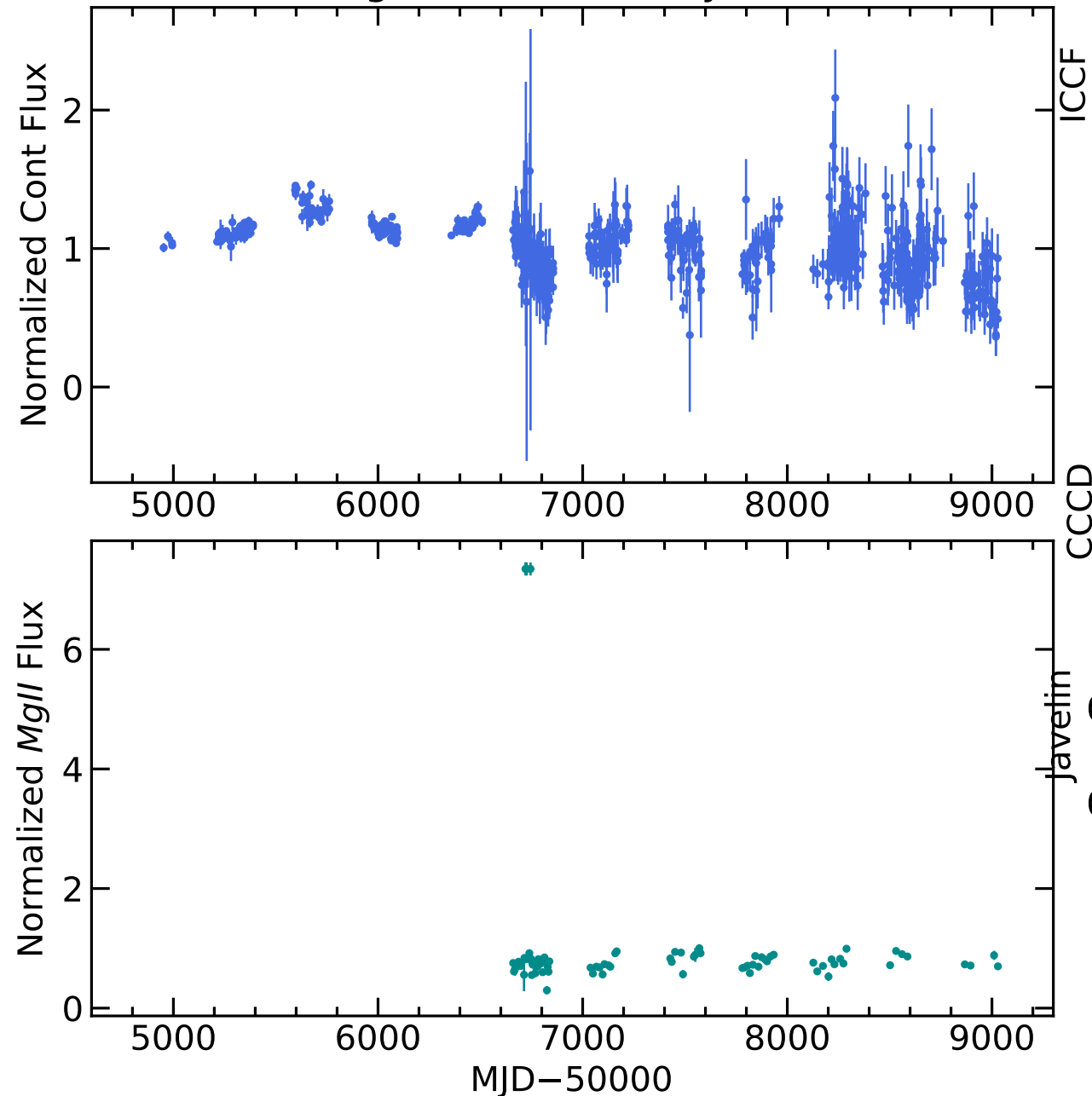
RM706 Light Curves (w/ PyROA model)
