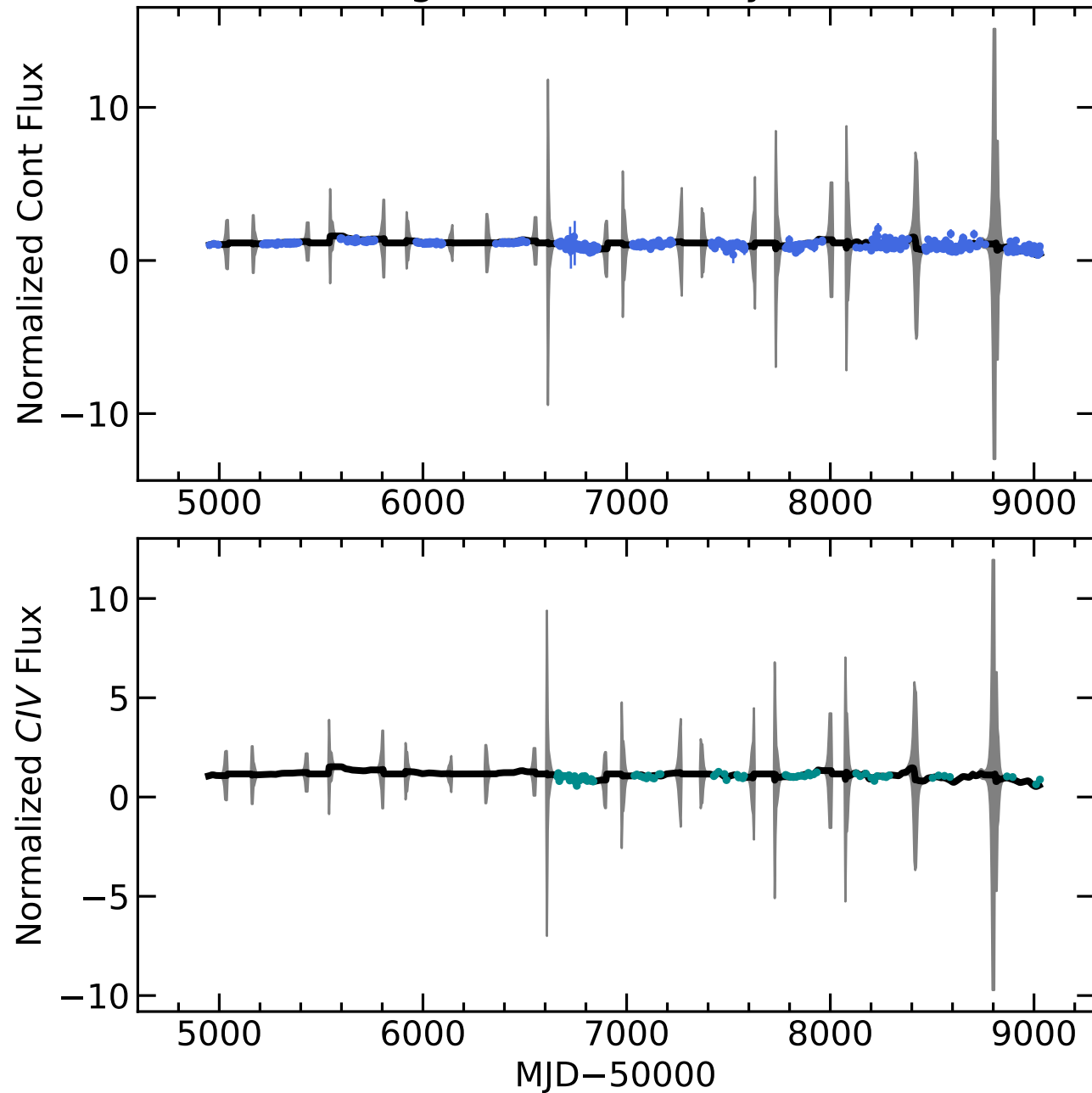
RM706 Light Curves (w/ PyROA model)
