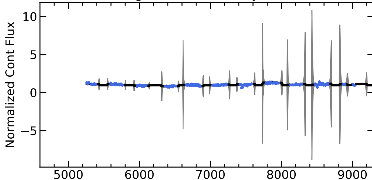
RM710 Light Curves (w/ PyROA model)
