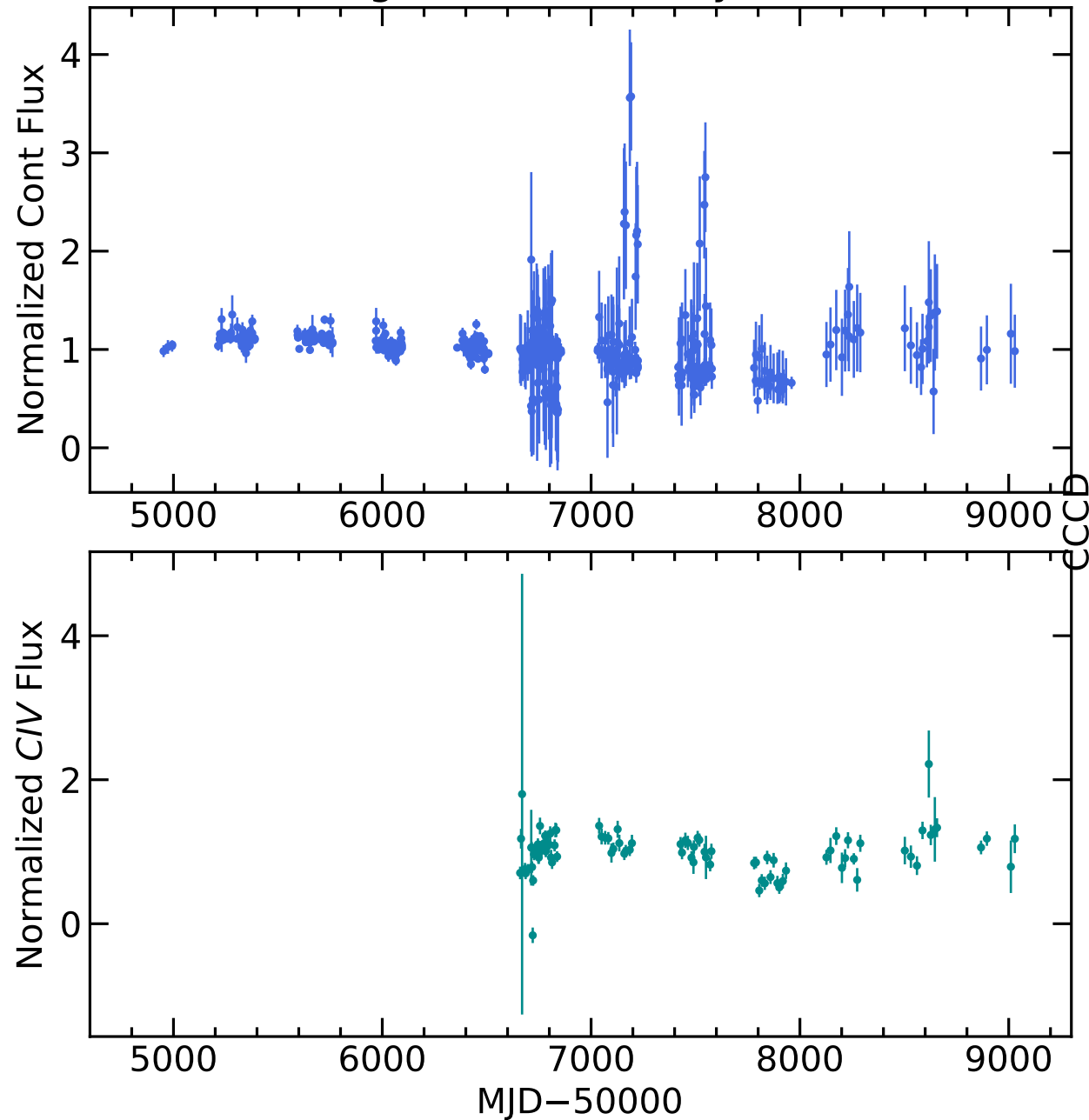
RM712 Light Curves (w/ PyROA model)
