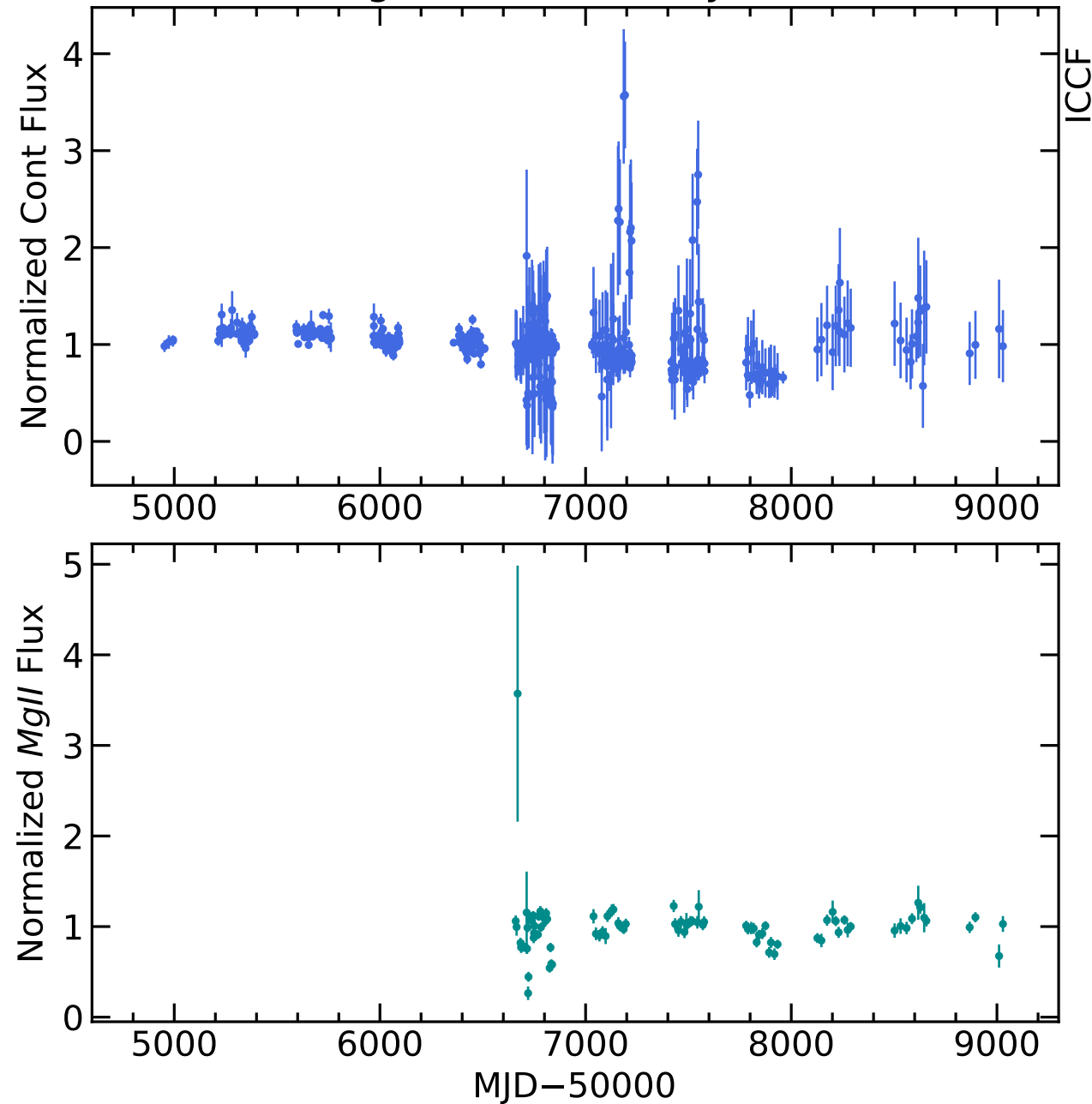
RM712 Light Curves (w/ PyROA model)
