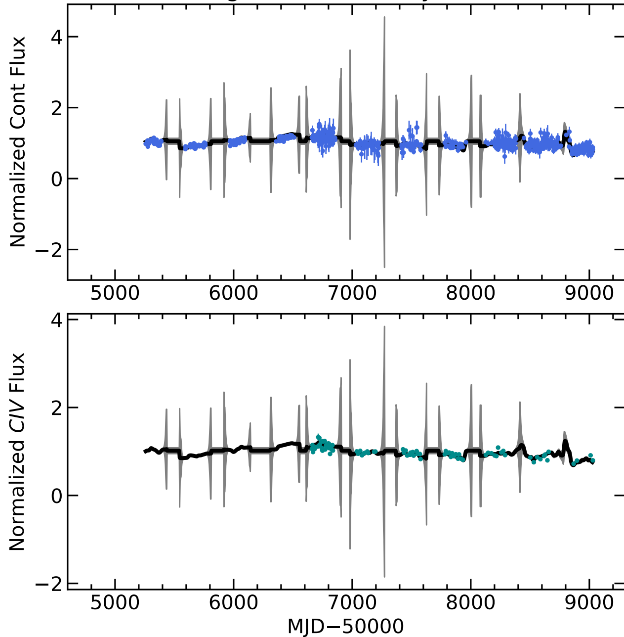
RM713 Light Curves (w/ PyROA model)
