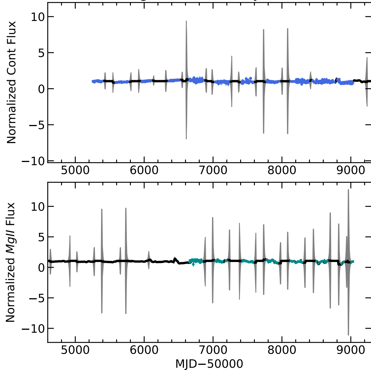
RM713 Light Curves (w/ PyROA model)
