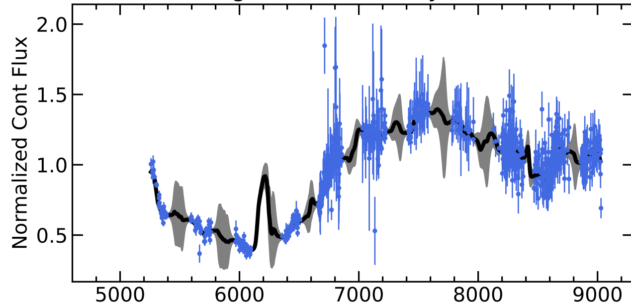
RM714 Light Curves (w/ PyROA model)
