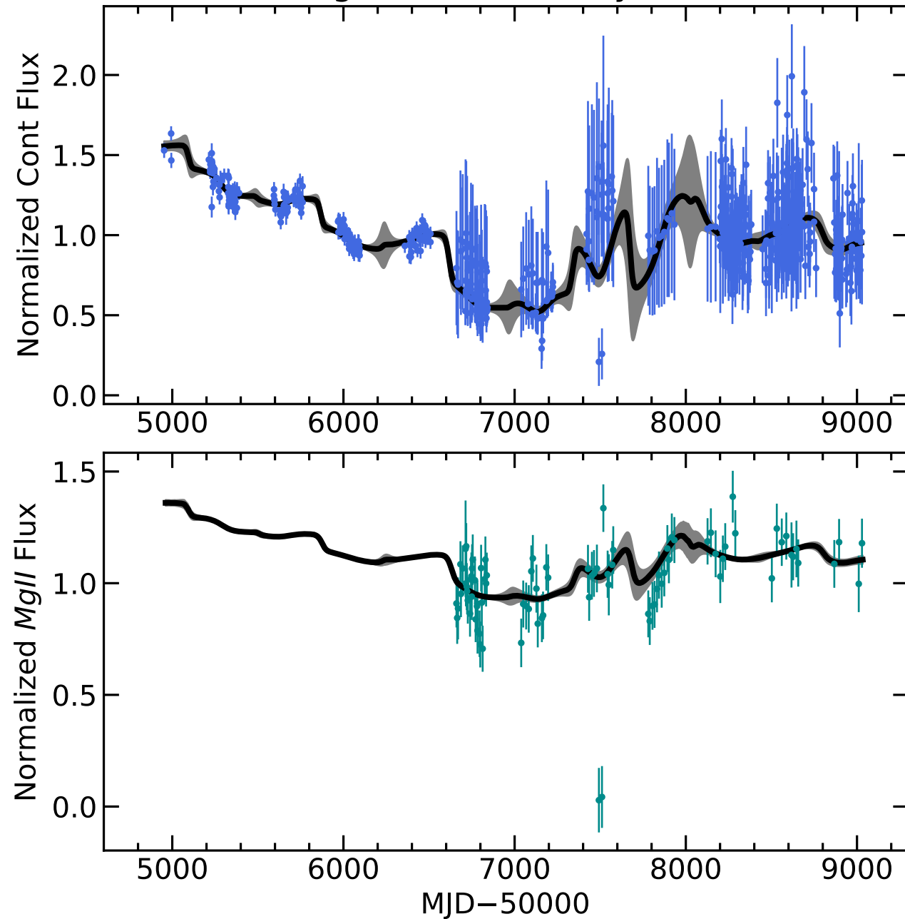
RM715 Light Curves (w/ PyROA model)
