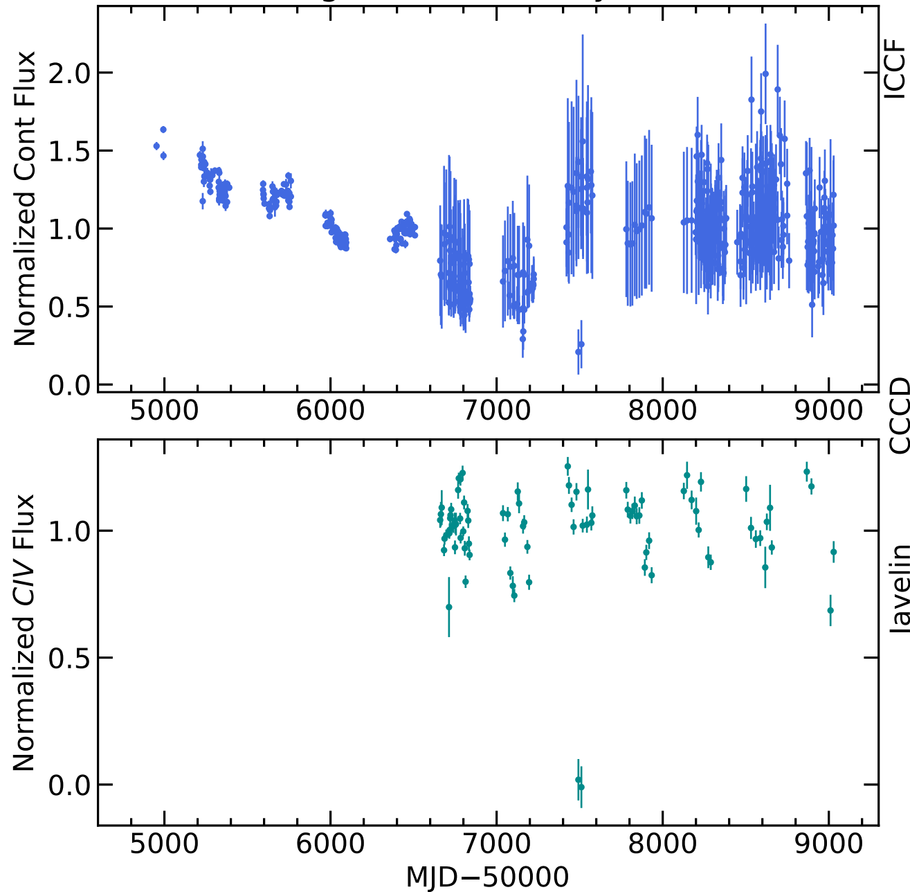
RM715 Light Curves (w/ PyROA model)
