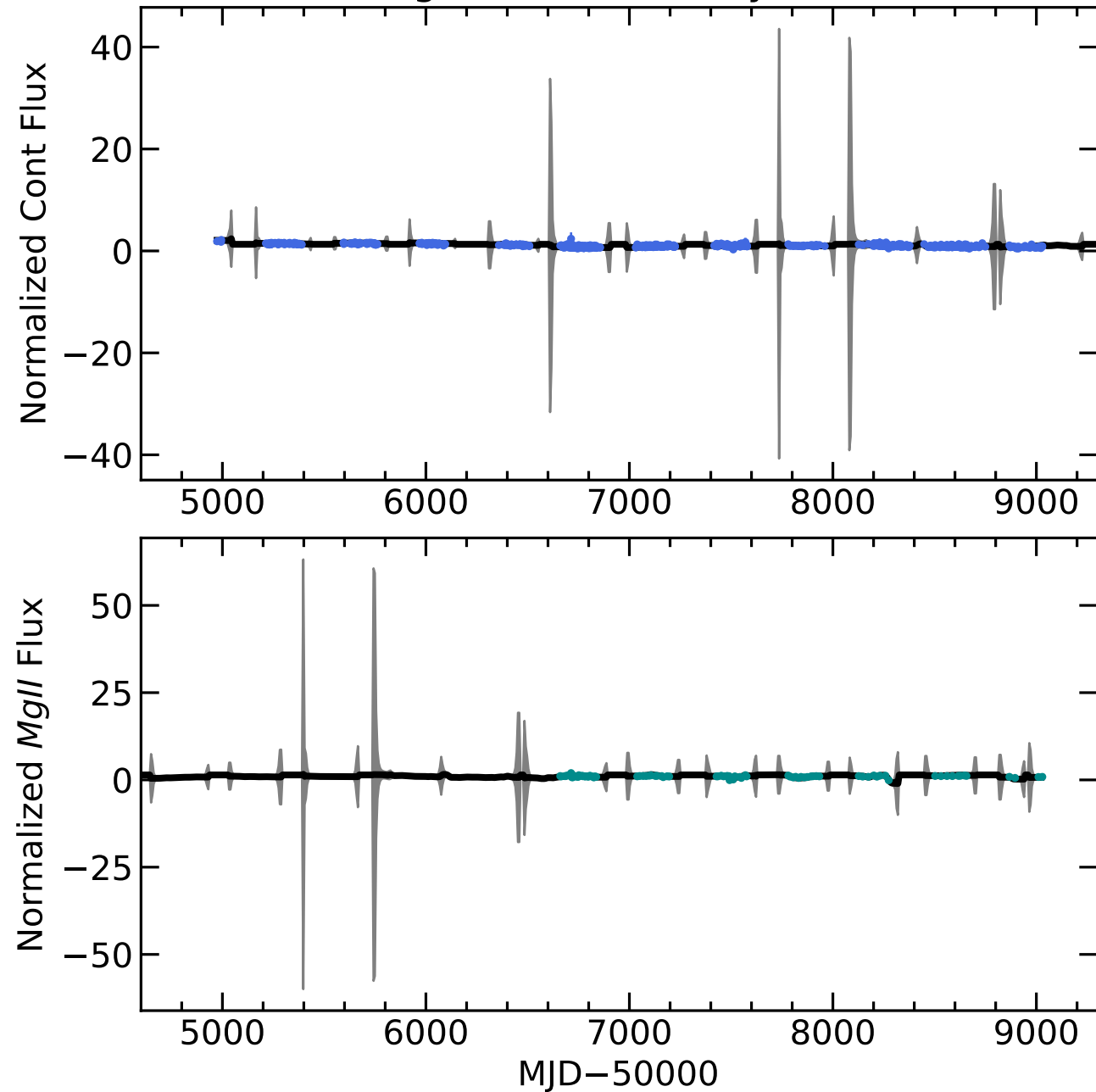
RM717 Light Curves (w/ PyROA model)
