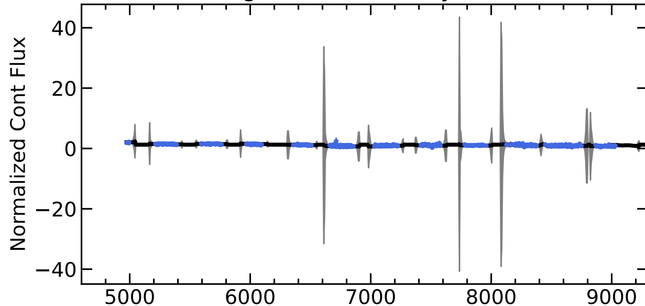
RM717 Light Curves (w/ PyROA model)
