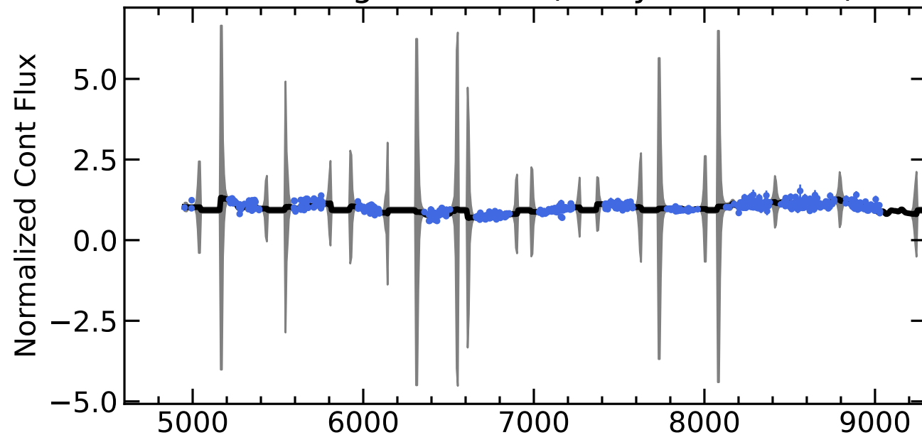
RM718 Light Curves (w/ PyROA model)
