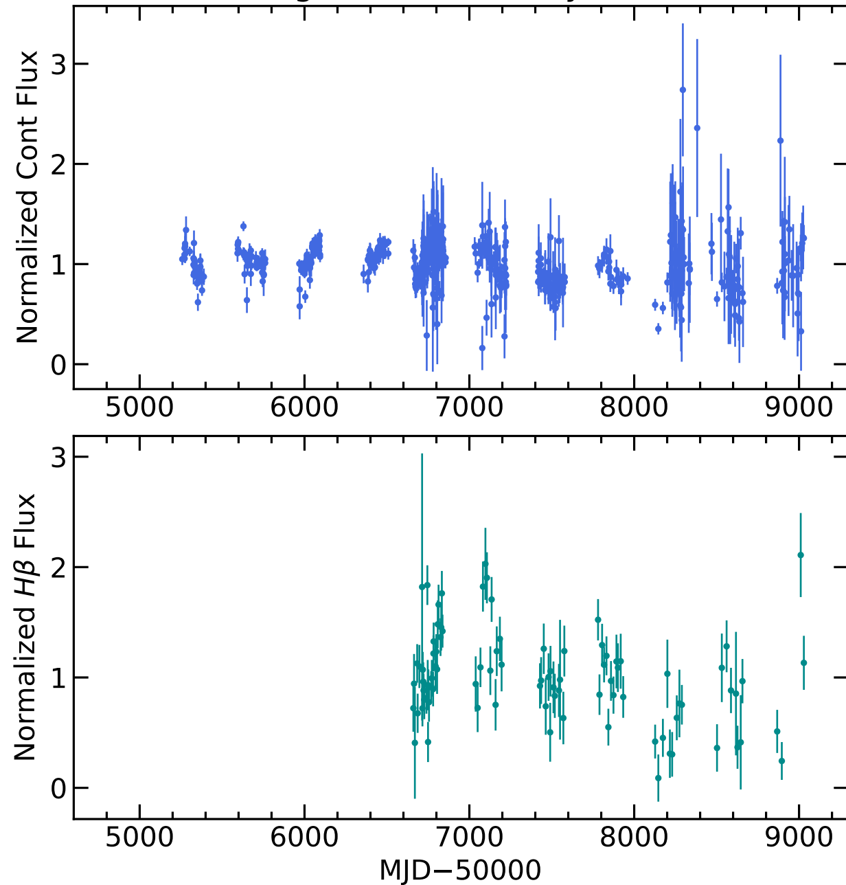
RM719 Light Curves (w/ PyROA model)
