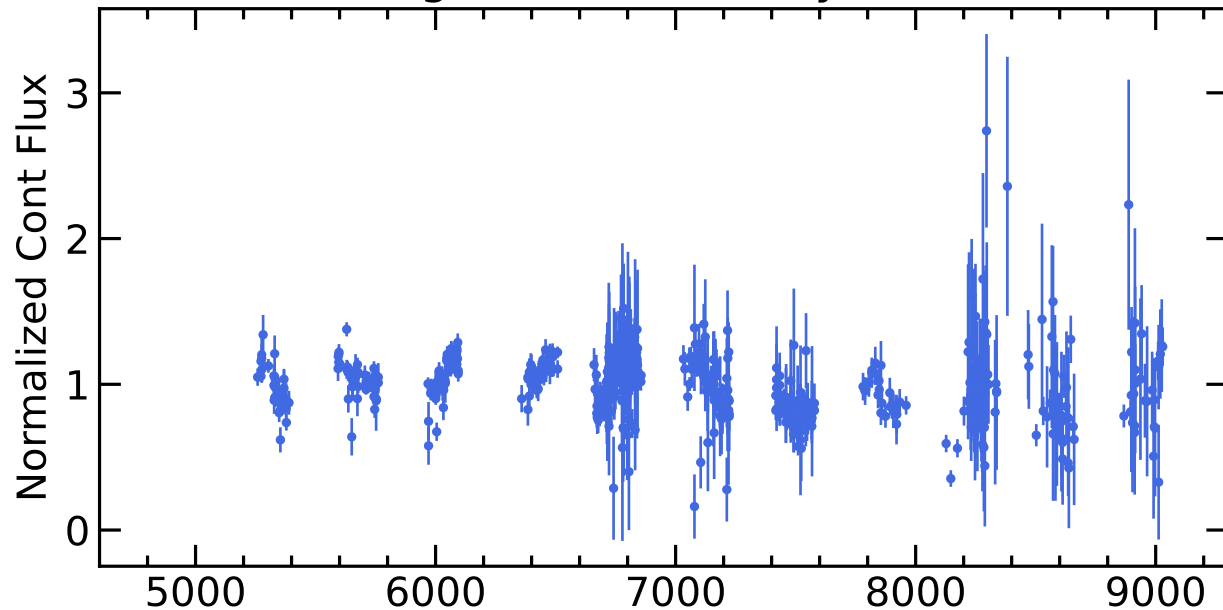
RM719 Light Curves (w/ PyROA model)
