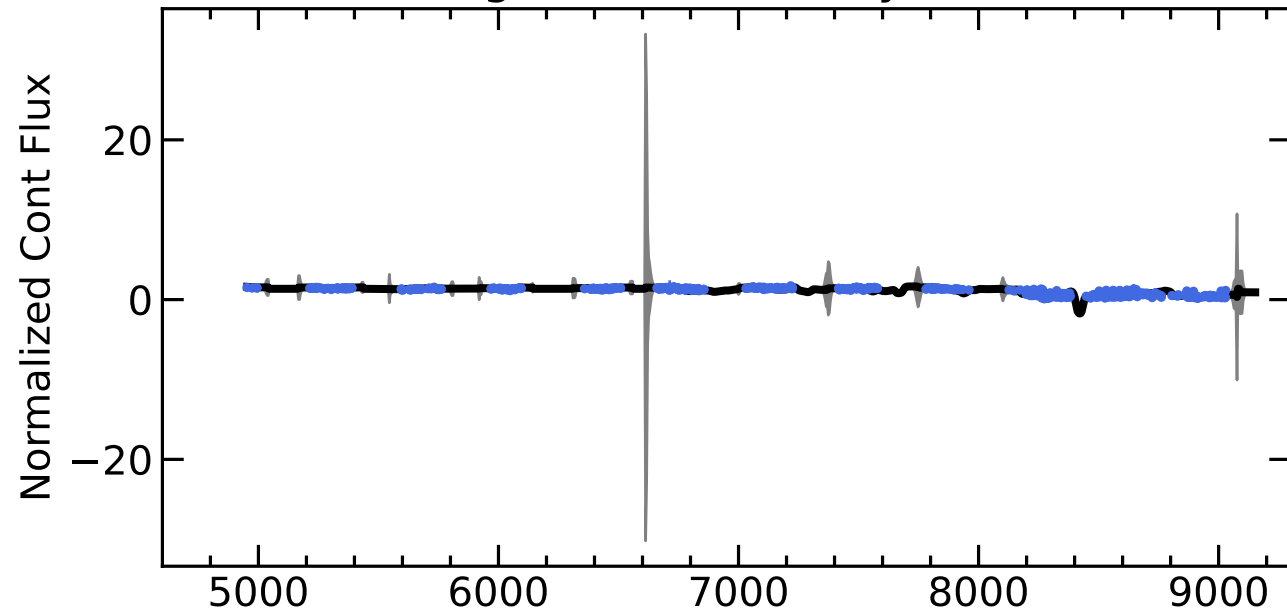
RM720 Light Curves (w/ PyROA model)
