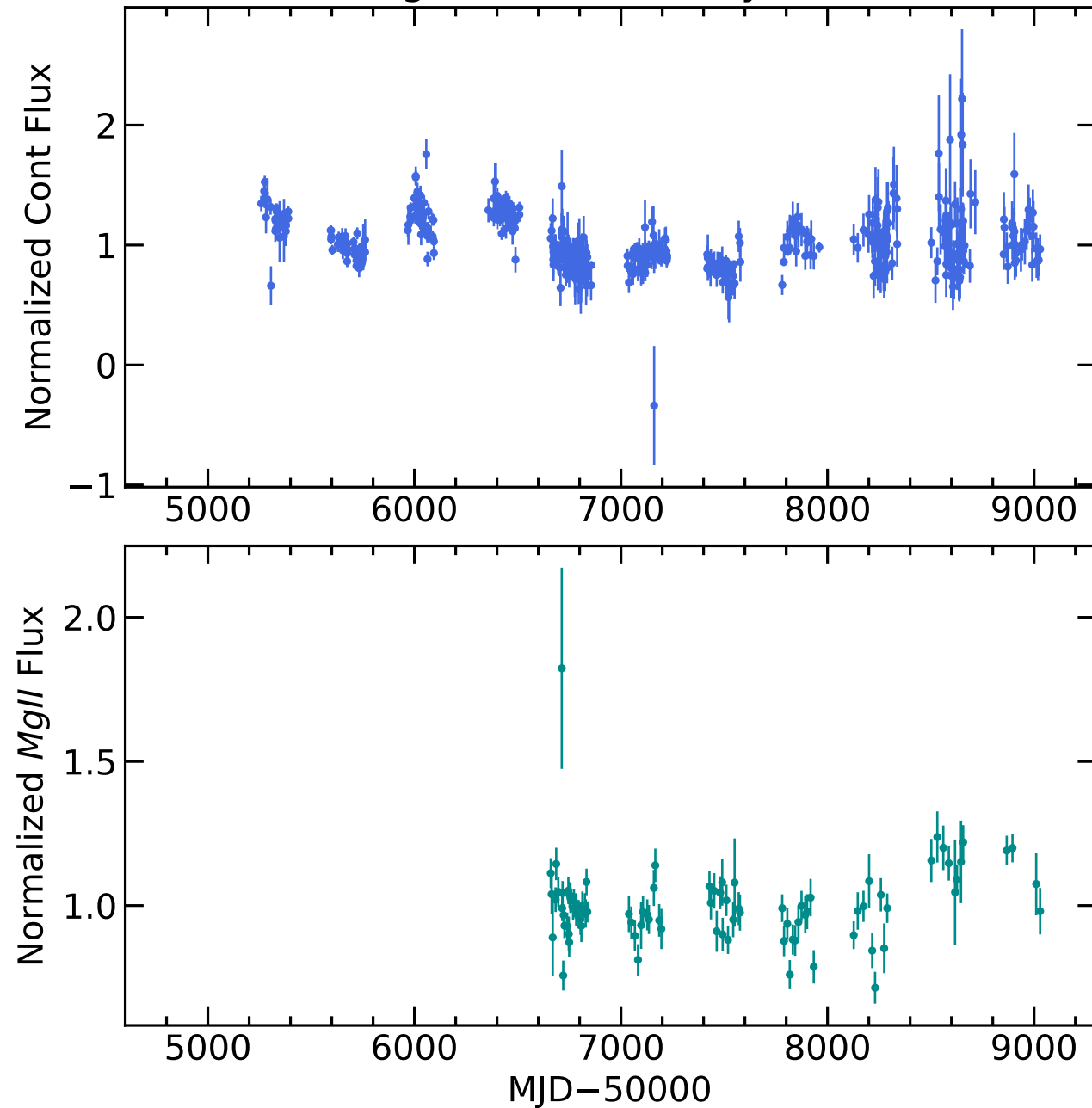
RM721 Light Curves (w/ PyROA model)
