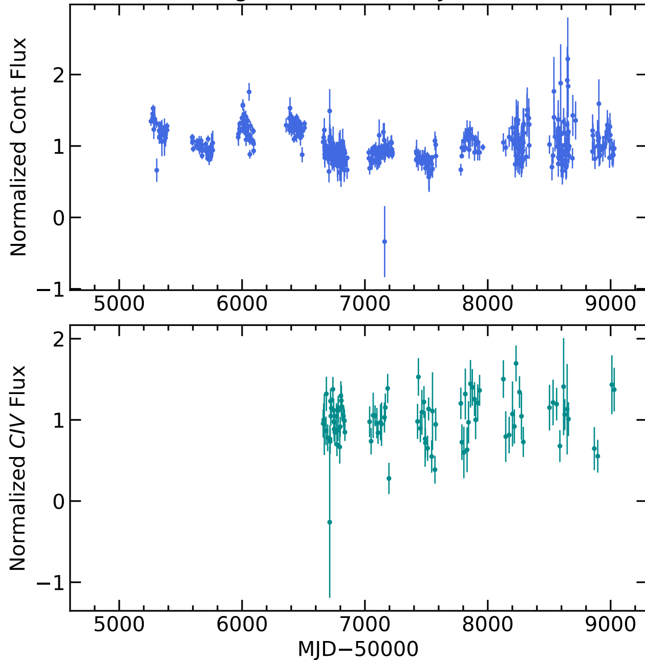
RM721 Light Curves (w/ PyROA model)
