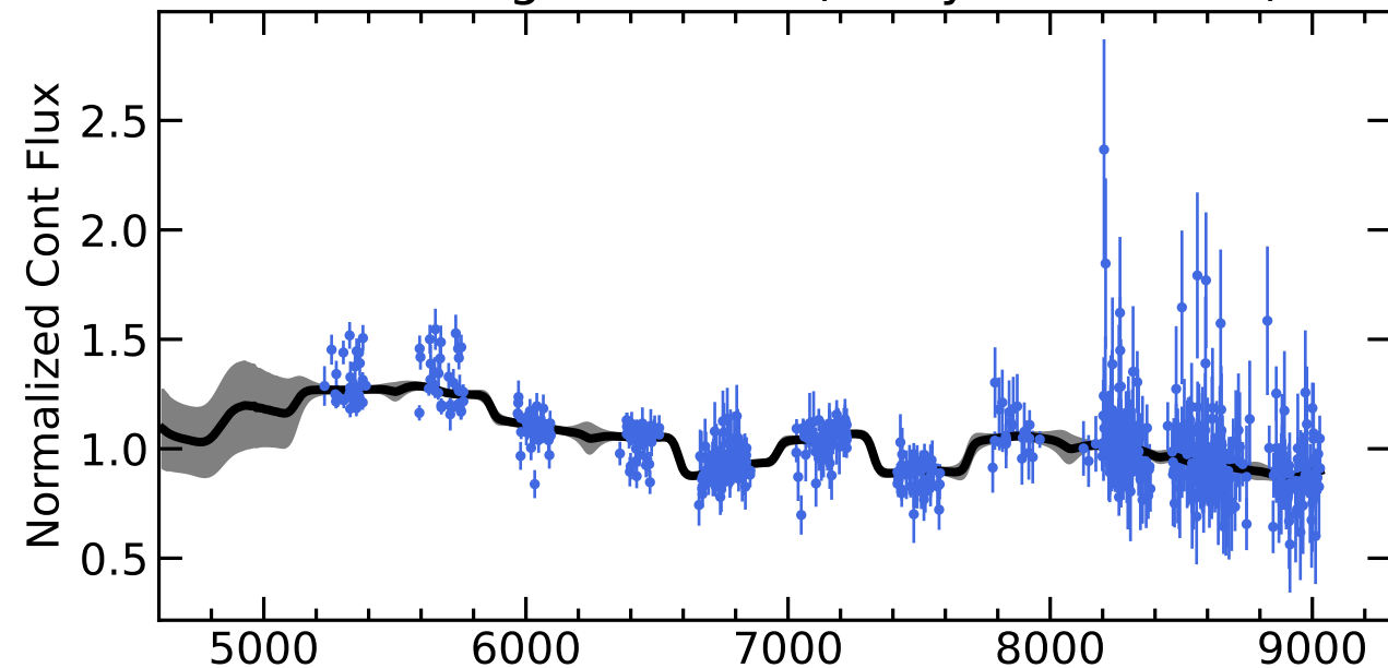
RM722 Light Curves (w/ PyROA model)
