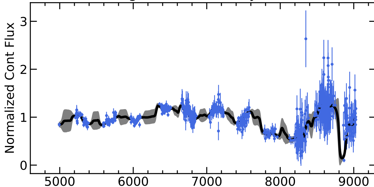
RM723 Light Curves (w/ PyROA model)
