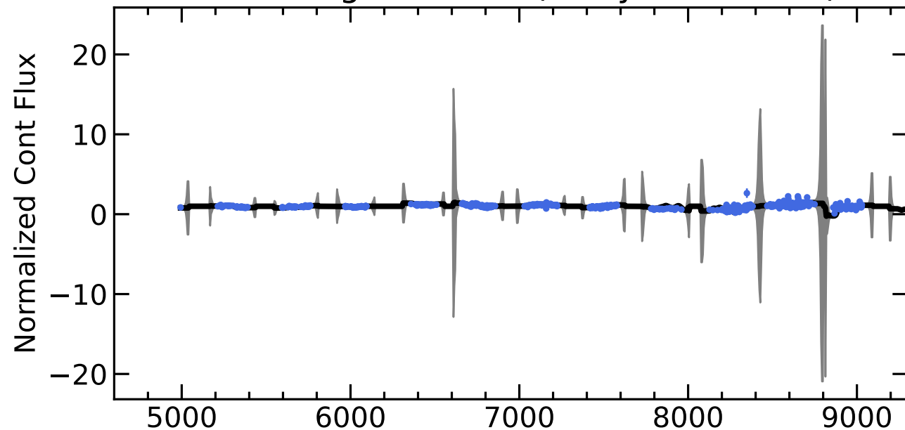
RM723 Light Curves (w/ PyROA model)
