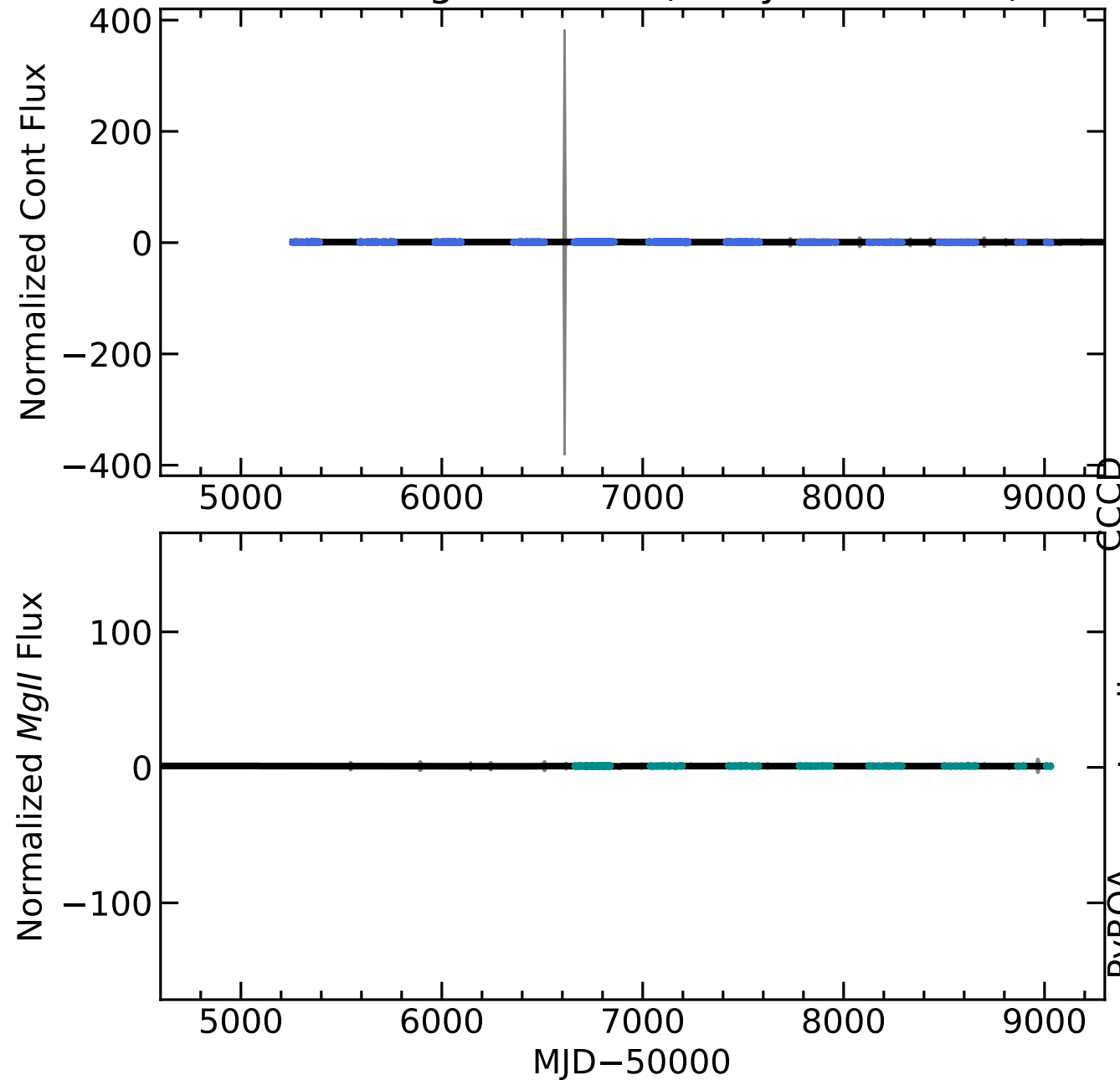
RM724 Light Curves (w/ PyROA model)
