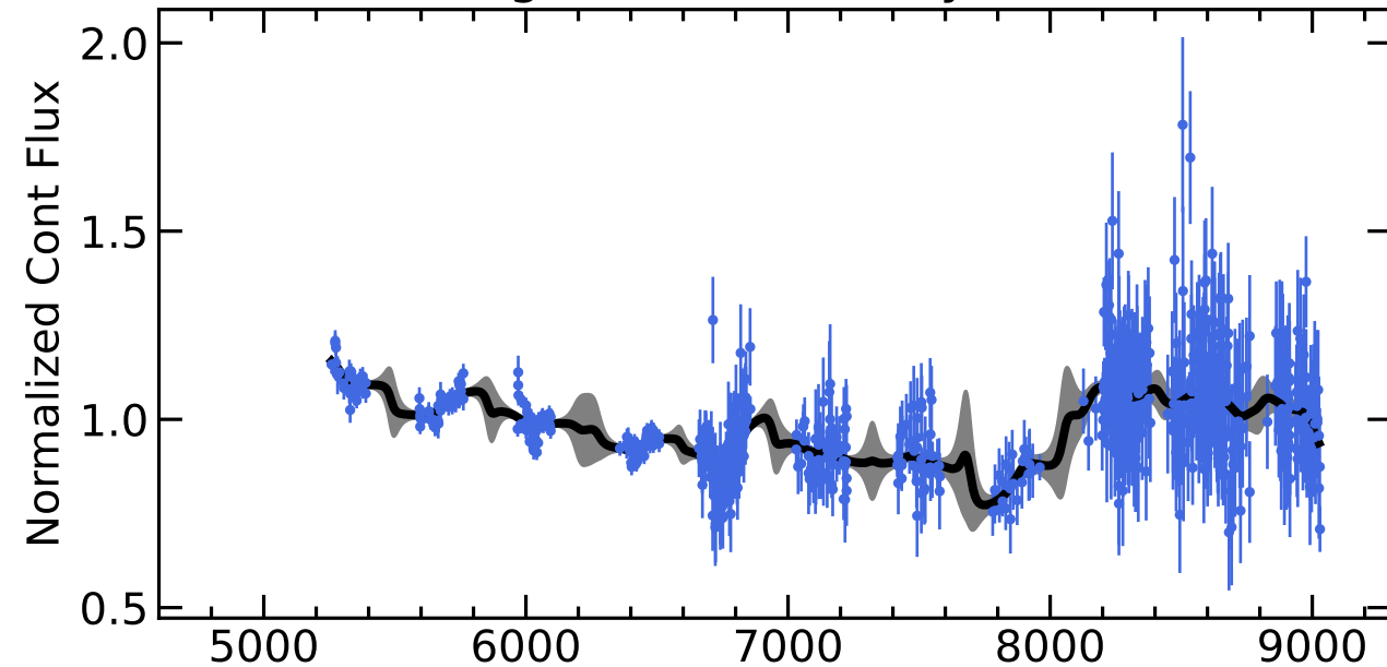
RM725 Light Curves (w/ PyROA model)
