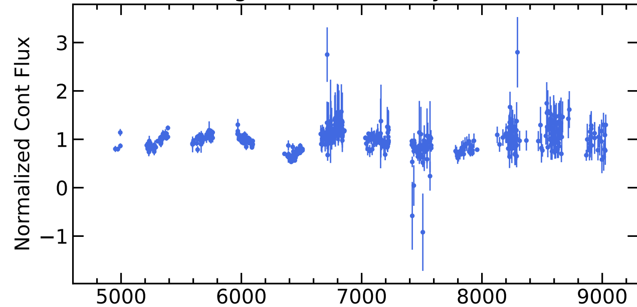
RM726 Light Curves (w/ PyROA model)
